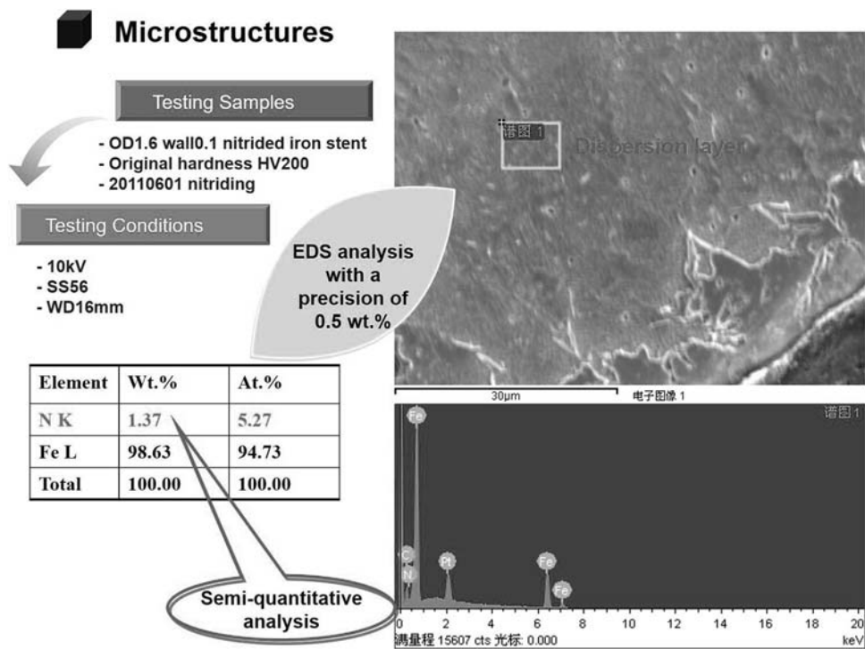
Figure S1: The SEM observation of the nitride iron surface and the corresponding EDS analysis.
