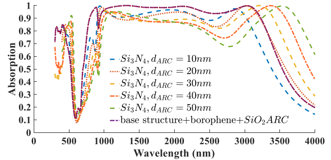
Figure 9: Absorption spectra of the borophene-based absorber using a \text{Si}_3\text{N}_4 ARC layer with varying thicknesses (10–50 nm). The results are compared to the optimal case with a 190 nm \text{SiO}_2 ARC layer.
