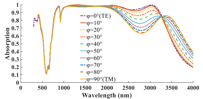
Figure 10: \phi dependent absorption response of the structure under \phi = 0 (TE) to \phi = 90 (TM) incidents.
