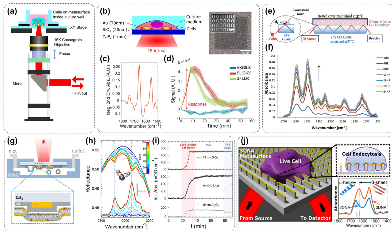
Figure 4: Metasurface for IR imaging of live cells. (a) Schematic drawing of the light path diagram for in vivo imaging of cells by infrared spectroscopic microscopy [72]. (b) Cells can efficiently adhere to the metasurface substrate, and (c) the signal amplification of the metasurface can facilitate the SEIRA measurement cellular response to (d) the activation of PAR1/PAR2 receptors by three synthetic peptides [72]. (e) A schematic diagram illustrates the multireflection ATR-FTIR measurement setup and (f) a representative set of ATR-FTIR spectra obtained from live MDA-MB-231 cells after a 24-h seeding period [73]. (g) A schematic representation depicting the fluidic chamber and experimental setup during measurements. The yellow and red phospholipid headgroups signify DOPC and Texas RED DHPE, respectively. (h) The vertical dashed lines indicate the spectral positions of the symmetric (depicted in blue) and asymmetric (depicted in red) CH 2 stretching modes and (i) the significant differences in the adsorption efficiency of phospholipids on different materials [79]. (j) IR spectroscopic detection of protein (including clathrin and AP-2 complex) conformational changes during clathrin-mediated endocytosis assisted by metasurface [42].
