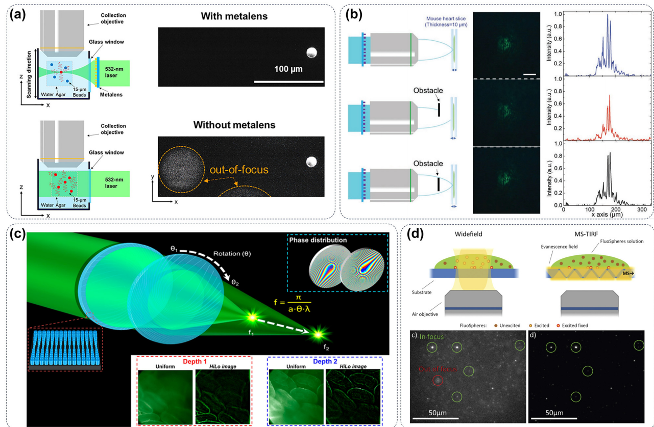
Figure 8: Metasurface improves the imaging ability of fluorescence microscopy. (a) The spatial resolution of a fluorescence microscope can be improved by embedding a GaN metasurface into the optical path of the microscope [127]. (b) Metasurface structures generate an abrupt autofocusing beam to improve the deep tissue imageability of fluorescence microscope [128]. (c) The moiré metalens consists of two complementary phase metasurfaces that eliminate the spherical aberration and distortion generated in the process of fluorescence microscope imaging [129]. (d) The metasurface facilitated the coupling of light into a microscopy coverslip, enabling the achievement of TIR excitation [130].
