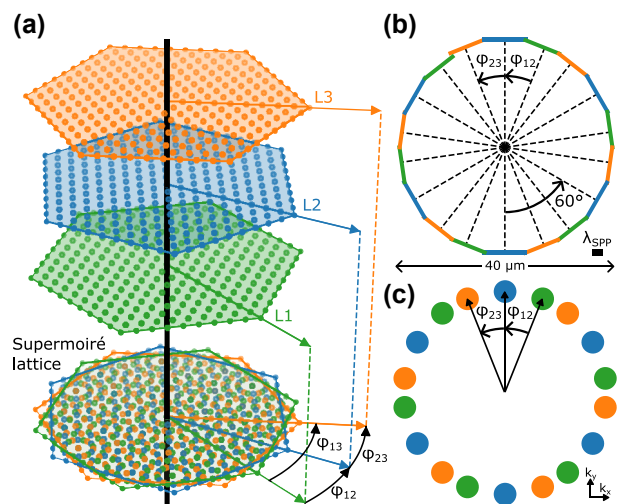
Figure 1: Plasmonic super-moiré skyrmion lattices. (a) Super-moiré lattice created by three hexagonal lattices with relative twist \phi_{12} between the first and second lattice (L1 and L2) and \phi_{23} between the second and third lattice (L2 and L3). In plasmonics, the lattices are superimposed in a single layer as illustrated at the bottom. (b) Corresponding coupling structure of a super-moiré skyrmion lattice. The coupling structure consists of three tilted hexagons, generating three skyrmion lattices with relative twists. (c) Schematic Fourier decomposition of a moiré skyrmion superlattice, where the colors originate from the boundaries in (b) and the lattice colors in (a).
