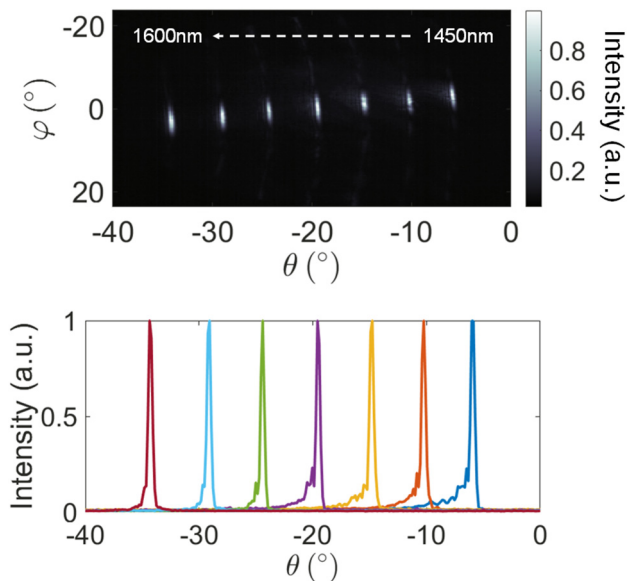
Figure 5: Demonstration of 2D beam-steering. Top: Superimposed far-field images for different optimized angles in \varphi -axis and \theta -axis. To steer in \theta , the wavelength is tuned from 1450 to 1600 nm. Bottom: Line cuts in \theta of the beams in the image above.
