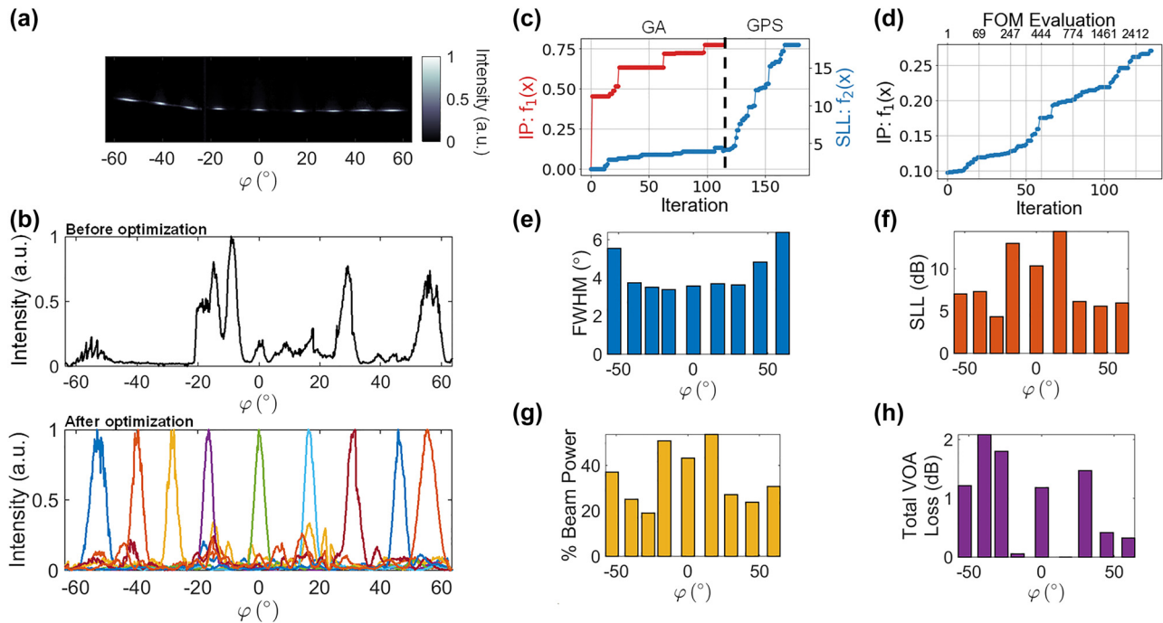
Figure 3: Measurement results for 9 steering angles. (a) Superimposed far-field images for different optimized angles in \phi -axis. Each beam is normalized to its maximum intensity (b) Top: OPA emission before optimization. Bottom: Elliptical line cuts of the optimized solutions shown in (a). (c) Figures of merit (FOM) at each iteration for forming a beam at 0^\circ without prior knowledge of existing beam solutions. A multi-objective genetic algorithm (GA) with a population size of 50 and a generalized pattern search algorithm (GPS) were used for the optimization. (d) FOM at each iteration for forming a beam at 55^\circ with the benefit of knowing the optimized values for a solution at 50^\circ . Only the pattern search algorithm was used for the optimization. For the various optimized angles measured: (e) FWHM, (f) sidelobe levels (g) % beam power: power in the main beam as a percentage of the total radiated power (h) total VOA loss: total radiated power normalized to the maximum observed radiated power across all measurements.
