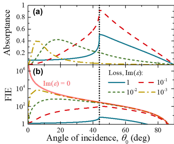
Figure 5: Angular dependence vs. varying ENZ loss. (a) Absorptance and (b) FIE of Mode 1 in an ultrathin ENZ film with a fixed thickness of 22 nm at the ENZ wavelength of 1627 nm ( \delta = 0.08 ). The varying loss is shown in the legend. In the calculations we use n_0 = 1.44 and n_s = 1 . The solid red semitransparent line in (b) shows the limiting case of infinitesimal ENZ losses of Eq. (13). The vertical dotted line is the critical angle of 43.8^\circ .
