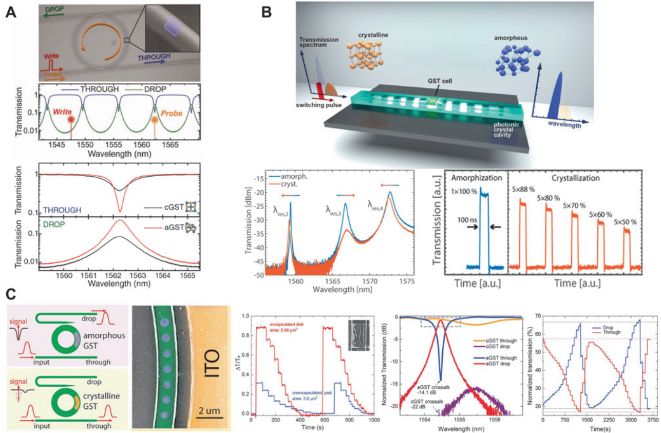
Figure 15: Fully integrated phase-change switches and modulators enabled by on-chip optical pulse triggers. (A) Top: Operation principle of an all-photonic integrated phase-change switch consisting of a GST element (inset) on top of a ring resonator which is evanescently coupled to two parallel waveguides. For the on-resonance condition (when the laser wavelength is equal to the resonance wavelength of the ring resonator), the power is divided between THROUGH and DROP ports, while for the off-resonance condition (the laser wavelength is detuned from the resonance wavelength of the ring resonator), all power is delivered to the THROUGH port. Therefore, to control the state of GST optically, the 'write' signal wavelength should be adjusted to that of the ring resonator (on-resonance condition). Bottom: Transmission spectra of the ring resonator in the THROUGH (upper panel) and DROP (lower panel) port showing that the on-resonance light is delivered to either the THROUGH port in the crystalline state (black curve) or DROP port in the amorphous state (red trace) [215]. (B) Top: Illustration of a reversible all-photonic switch consisting of a photonic crystal cavity waveguide integrated with a GST cell evanescently coupled to the center of the cavity. Bottom left: The change in both transmission and spectral position of the resonance modes of the cavities due to phase transition of GST. Bottom right: The switching scheme used for amorphization (using a single 100 ns optical pulse with 100% peak power) and re-crystallization (using five groups of pulses with decreasing energy, in which each group contains five pulses with an identical peak power) [220]. (C) Left: Operation principle and the false-colored SEM image of the 1 \times 2 optical switch working based on optically induced phase transition of the seven subwavelength GST nanodisks patterned on a SiN microring resonator. Right (left panel): The stepwise change in the optical transmission of a simple SiN waveguide covered by five GST nanodisks (the structure is not shown here) as the phase of the GST nanodisks changes using optical pulses. Multiple transmission levels are achieved by step-wise re-crystallization of the encapsulated GST nanodisks area (red) and the unencapsulated unpatterned GST patch (blue) (inset: SEM image of the GST patch deformed after one optical pulse). Right (middle panel): The transmission spectra at the through and drop ports of the 1 \times 2 optical switch near a resonance of the microring resonator when the phase of GST changes from amorphous (high (low) transmission at drop (through) port) to crystalline (redshifted high (low) transmission at through (drop) port). Right (right panel): Transmission spectra achieved from the drop and through ports upon amorphization (set) using optical pulses and stepwise re-crystallization (reset) using electrical pulses applied to the ITO heater. Up to 20 intermediate transmission levels are achieved enabling multilevel switching [211].
