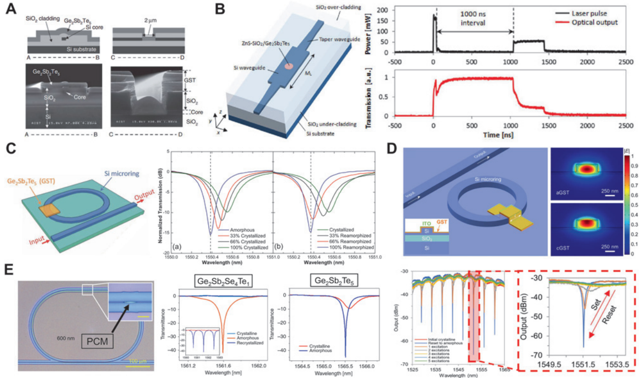
Figure 14: Photonic integrated phase-change switches and modulators triggered with free-space illuminations. (A) The schematic (top) and SEM images (bottom) of the pioneering work on one-way (left) [218] and reversible (right) [219] optical gate switching. (B) Left: Schematic of the optical gate switch consisting of a 1 \times 1 MMI waveguide with a circular-shaped GST cell on top excited by external out-of-plane laser pulses. Right: The waveforms of laser pulses (upper diagram) and optical transmission at output (lower diagram) with a sequence of OFF/ON/OFF operations [207]. (C) Left: A reversible optical switch consisting of a Si racetrack resonator (partially deposited by a thin film of \text{Ge}_2\text{Sb}_2\text{Te}_5 ) coupled to a Si waveguide. Middle and right: The evolution of the transmission spectrum during crystallization (middle) and re-amorphization (right) showing the reversible switching operation [208]. (D) Left: Schematic of the GST-on-Si photonic modulator (inset: cross-section of the hybrid waveguide). Right: The mode profiles of the hybrid waveguide at 1550 nm for amorphous (top) and crystalline (bottom) states. Bottom: Transmitted output spectra of the modulator employing a 2 \mu\text{m} width GST element excited with a train of pulses with different pulse numbers [210]. (E) Left: Optical image of the resonant switch in which a low-loss GSST nanostrip deposited on top of a SiN ring resonator as shown in the inset. Middle and Right: The transmission spectra of the switch showing complete ON/OFF modulation of the resonant peaks when integrated with \text{Ge}_2\text{Sb}_2\text{Se}_4\text{Te}_1 (middle) outperforming the traditional resonant switch with the similar configuration but integrated with \text{Ge}_2\text{Sb}_2\text{Te}_5 (right) [122].
