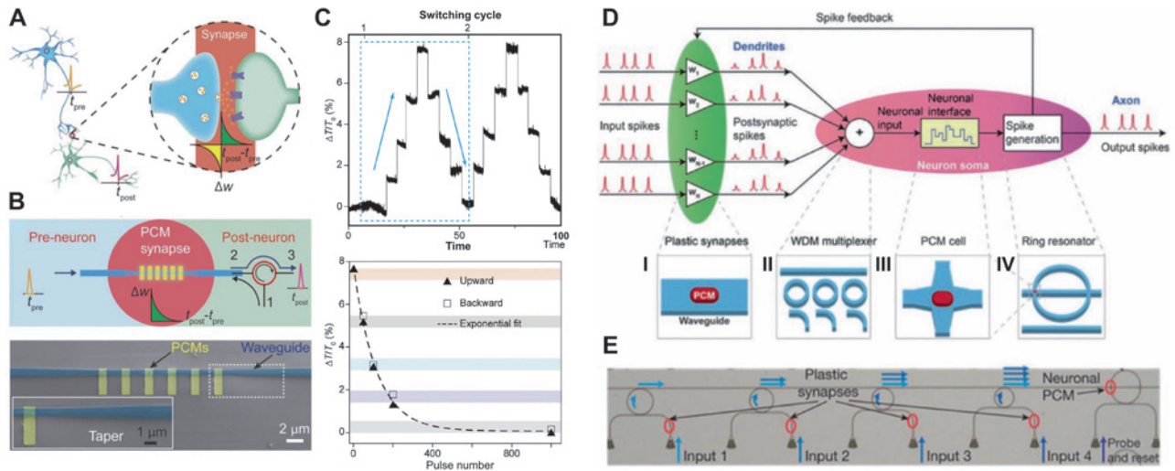
Figure 20: All-photonic fully integrated phase-change synapse and neuromorphic processor. (A) Conceptual representation of neurons and synapses. The inset shows a synapse junction and synaptic plasticity ruled by STDP, i. e., \Delta w = Ae^{-\Delta t/\tau} , in which \Delta t = t_{\text{post}} - t_{\text{pre}} , where A and \tau are constants [241]. (B) Schematic of an on-chip integrated photonic synapse consisting of a tapered waveguide (dark blue) covered by discrete GST islands (yellow). GST islands are initially crystalline (i. e., T_0 = '0' ). Change in the transmission level (i. e., \Delta T/T_0 ), by modifying the crystallization level of GST, is attributed to the synaptic plasticity of the device ( \Delta w ). \Delta T/T_0 can be controlled by the number of triggering pulses similar to those in the STDP in the neural synapse shown in A [241]. (C) Top: Five optical transmission levels of the devices related to the five weights of the photonic synapse which are obtained by optical pulses with 50 ns duration and 404.5 pJ energy. Bottom: The dependency of the synaptic weight ( \Delta T/T_0 ) to the number of pulses which can be fitted by an exponential fitting function of \Delta T = Ae^{r \times N} to resemble the STDP in a neural synapse shown in A [241]. (D) Top: Schematic of the all-photonic neurosynaptic system implemented in [242] comprising of N pre-synaptic neurons (generating pre-synaptic spikes) and one output neuron (the red region) which interconnected by N synapses (green region). Bottom: The input spikes are weighted by plastic synapses (I), and combined and directed into an output waveguide using the WDM technique (II), and fed into a PCM cell (III) on a large ring resonator (IV) mimicking the biological neural functionality of an actual neuron. (E) Optical microscope image of a fabricated neuron in which four inputs are weighted by four synapses and coupled to four small ring resonators to be delivered to the output waveguide [103, 242].
