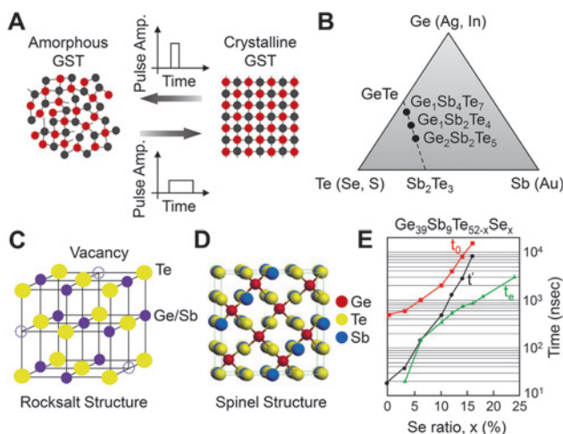
Figure 1: Principles of phase transformation in GST-based PCMs. (A) Schematic illustration of the reversible switching of the GST phase between amorphous and crystalline states. A long pulse with a moderate amplitude enables amorphous-to-crystalline conversion. A short pulse with a large amplitude enables crystalline-to-amorphous conversion via the melt-quenching process. (B) The phase diagram of the Ge–Sb–Te system. The dashed line shows the pseudo-binary line, which connects GeTe and \text{Sb}_2\text{Te}_3 compositions. Most popular GST-based PCMs can be identified on this line. (C, D) Rocksalt (cubic) and spinel structures of GST with octahedral and tetrahedral Ge coordination, respectively. As shown in C, most GST-based PCMs contain up to \sim 25\% vacancy-type defects at Ge/Sb sites. (E) Role of Se doping in modifying the switching mechanism (hence, speed) of a representative GST alloy. t_0 : nucleation time of as-deposited film, t' : nucleation time of the pre-conditioned film, and t_c : time needed for the full crystallization of the film. Panels (C–E) are adopted from [114], [115], and [116], respectively.
