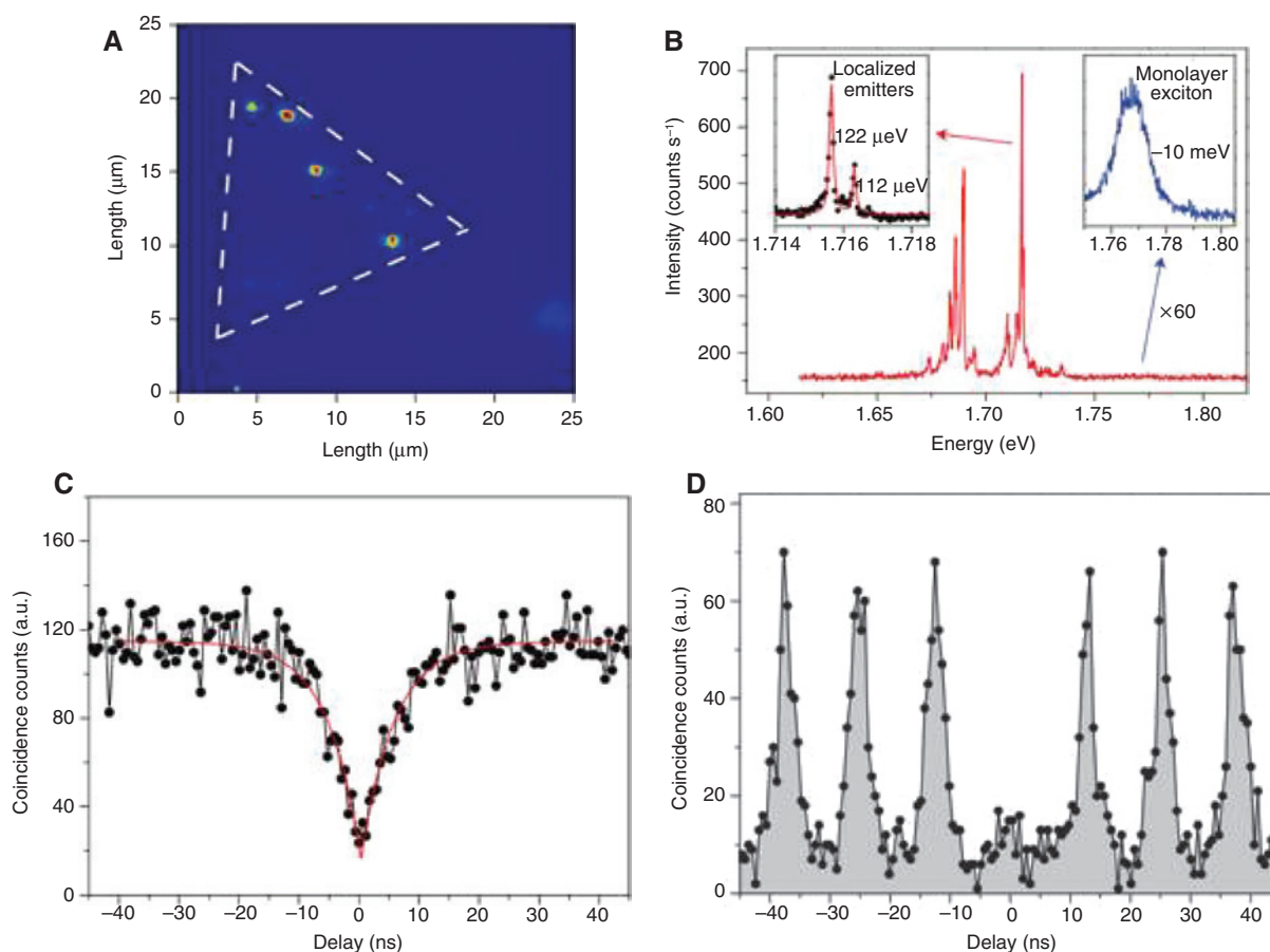
Figure 9: Single quantum emitters in layered materials. (A) Photoluminescence intensity map of narrow emission lines over 25\ \mu\text{m} \times 25\ \mu\text{m} area. The dashed triangle indicates the position of the monolayer; (B) photoluminescence spectrum of localized emitters. The left inset is a high-resolution spectrum of a defect emission. The right inset is a zoom-in of the monolayer valley exciton emission; observation of photon anti-bunching with (C) CW and (D) pulsed excitation. The dip at zero time-delay indicates presence of single photons. This figure is reprinted from Ref. [111].
