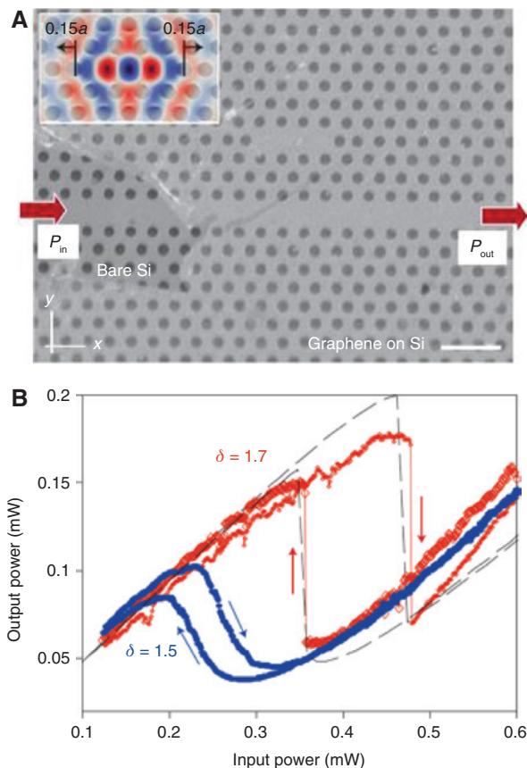
Figure 5: Optical bistability with graphene-clad silicon photonic crystal cavity. (A) Scanning electron micrograph (SEM) of the graphene-clad photonic crystal cavity; (B) output power as a function of the input power clearly shows the signature of optical bistability. The figures are reprinted from Ref. [85].
