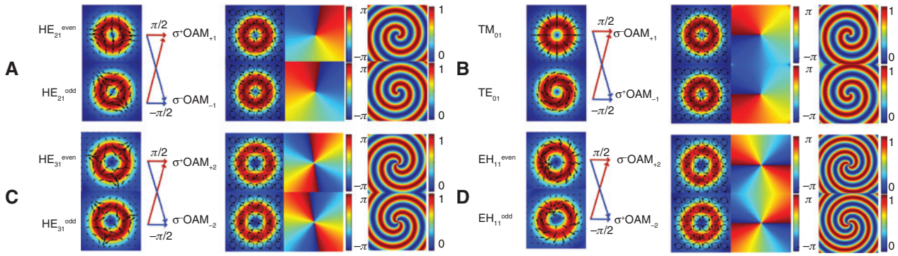
Figure 1: Intensity, polarization, phase, and interferogram of the \sigma^+OAM_{+1} (A), \sigma^-OAM_{+1} (B), \sigma^+OAM_{+2} (C), and \sigma^-OAM_{+2} beams (D).
