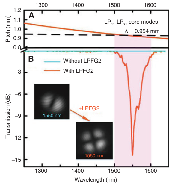
Figure 6: Calculated grating pitches against the resonant wavelength for the mode coupling from \text{LP}_{11} core mode to \text{LP}_{21} core modes (A); measured transmission spectra of LPFG2 with a period of 0.954 mm and a grating number of 40, and mode profile of the output 4MF at 1550 nm with and without LPFG2, respectively (B).
