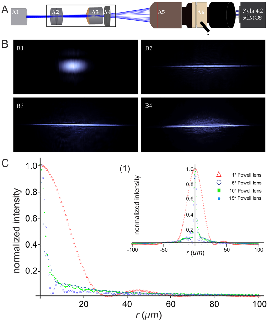
Figure 1: Effect of the fan angle of different Powell lenses on the intensity distribution of an incident Gaussian laser beam. (A) Experimental setup for measuring intensity distributions: (A1) 488 nm Sapphire laser with 200 mW power (Coherent Inc., Germany), (A2) Neutral Density Filters (NDFs, Thorlabs, USA), (A3) Powell lens with a fan angle of either 1°, 5°, 10°, or 15°, (A4) achromatic convex lens for guiding the altered beam into the entrance pupil of the detection objective without truncation, (A5) detection objective (Olympus XOL Fluor 4X, NA 0.28, WD: 29.25 mm, Japan), (A6) 3-position Trinocular Head U-TR30-2 (Olympus, Japan) with attached C-mount adapter connected to a Zyla 4.2 sCMOS camera (Andor, UK). (B) Transversal intensity distributions ( XY plane) of Gaussian laser beams after passing through Powell lenses with different fan angles. (B1–B4) demonstrate the beam profiles altered by passing through Powell lenses of 1°, 5°, 10°, and 15°, respectively. (C) The 2D-beam distributions (related to the thinness of the light distribution along the Y -axis of reshaped laser beams depicted in (B)), were measured over a range of \pm 100 \mu\text{m} away from the beam waist. For better clarity and precision (C) only shows one-half of the intensity distribution. The Inlay (1) represents the entire profile.
