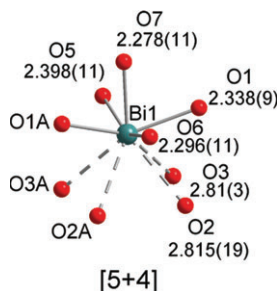
Figure 2 Oxygen coordination environment of the bismuth atom in the title compound. Symmetry transformations used: A=x, 0.5-y, z . Atomic positions of O2 and O3 are slightly disordered and have an occupation factor of 0.5 (Bi(1)–O(2'): 2.74(2) Å; Bi(1)–O(3'): 2.88(2) Å).
