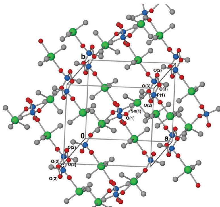
Figure 2 Unit cell of [\text{SnMe}_3\text{PhPO}_3\text{H}]_n showing intermolecular \text{P}=\text{O}\cdots\text{OH} hydrogen bonds. The phenyl groups have been omitted for clarity.
