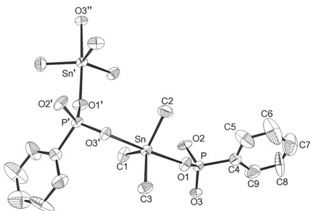
Figure 1 Zigzag infinite chain of [\text{SnMe}_3\text{PhPO}_3\text{H}]_n . H atoms and the second component of the disordered phenyl ring have been omitted for clarity. Symmetry codes: (') 1/2-x, y-1/2, 1/2-z (") x, y-1/2 ; displacement ellipsoids are drawn at the 50% probability level.
