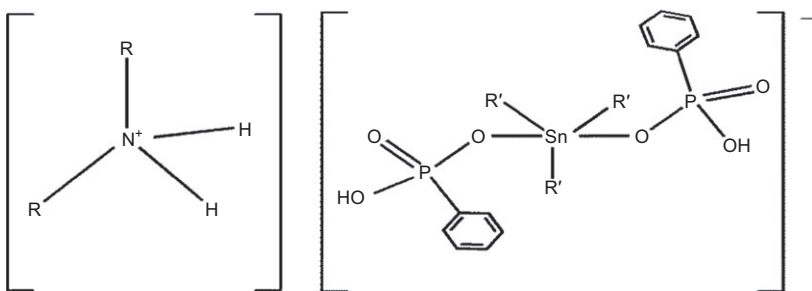
Scheme 1: Structure of \text{R}_2\text{NH}_2(\text{PhPO}_3\text{H})_2\text{SnR}'_3 ( \text{R}=\text{Cy}, \text{Bu} ; \text{R}'=\text{Me}, \text{Ph} ) ( 2 and 3 ).
