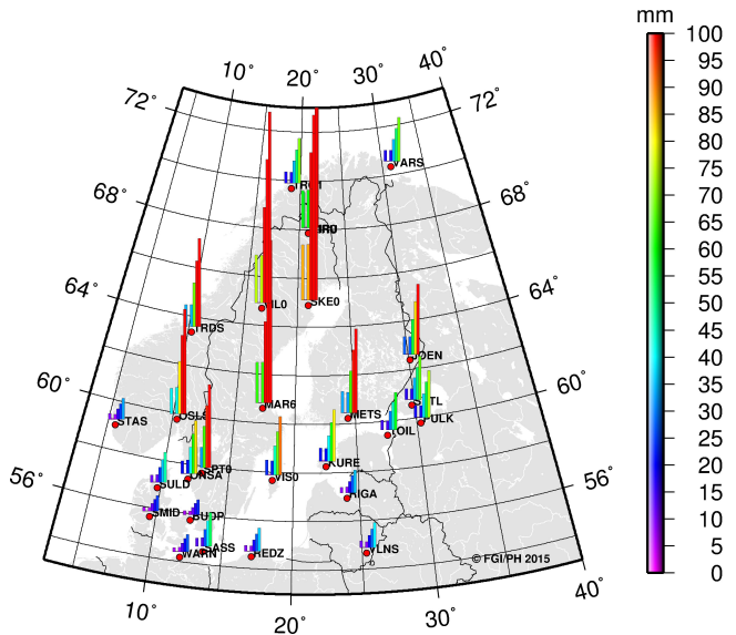
Figure 8: Coordinate difference ETRF2000(t) minus EPNC1785 in ETRF2000 at the epoch 2000.0 when IGB08 coordinates of the EPNC1785 are first converted with the station velocities to epochs 1990, 2000, 2010, 2020, 2030 and 2040 and then transformed with the standard EUREF transformation to the ETRF2000. Error bars from left to right show the difference for epochs 1990–2040.
