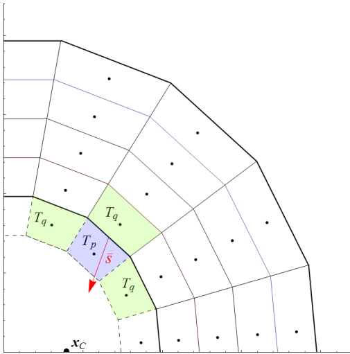
Figure 2: Illustration of the 2D FVM grid. The dashed lines denote the boundaries of added finite volumes, the volume of interest is shown in blue and its neighboring volumes in green. The vectors \vec{s} are depicted by red.
