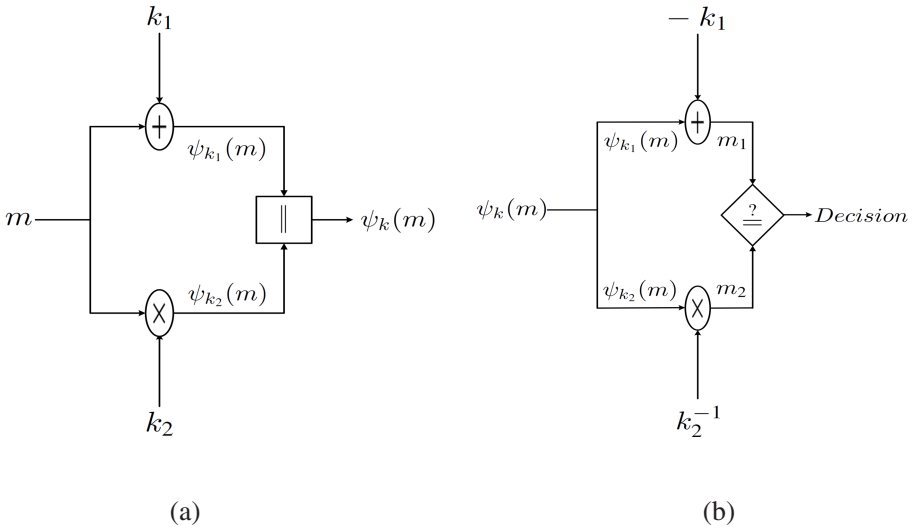
Figure 1. (a) A block diagram to implement the authenticated encryption scheme, and (b) A block diagram implementing the decryption and the validity check of the studied scheme. The addition and multiplication operations are performed over the ring \mathbb{Z}_n .
