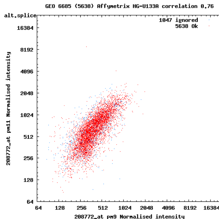
Figure 6: A scatter plot of the log 2 intensities between perfect match probes 9 and probe 11 from probeset 208772_at, obtained from 5638 HG-U133A GeneChips. For this particular probe pair, 1047 of the original set of 6685 chips were flagged as possibly providing spurious signals or being close to dubious values.
