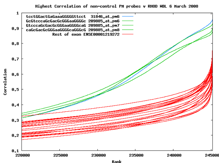
Figure 14: Rank of correlations between each of the probes mapping to exon ENSE00001219272 and the rest of the probes on the GeneChip HG-U133Av2. The several thousand probes that show close correlation have runs of contiguous guanines. We suggest this signal comes from probe-probe interactions resulting in G-quadruplexes.
