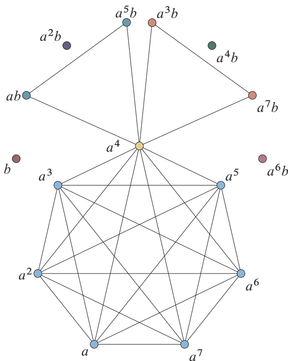
Figure 1. \mathcal{P}^*(QD_{16}) : vertices with different colours are in distinct N -classes.
