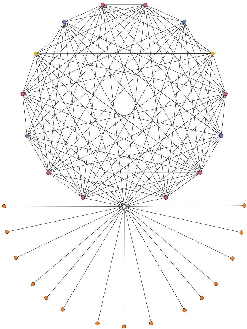
Figure 2. \mathcal{P}(\mathcal{D}_{30})
