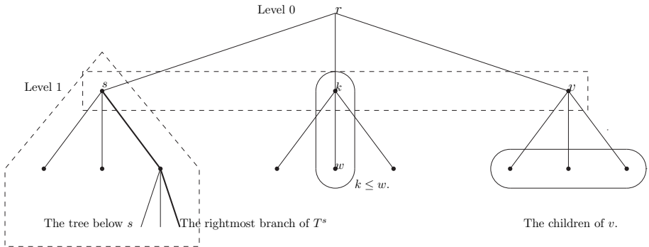
Figure 1. Levels, children, and trees below vertices
