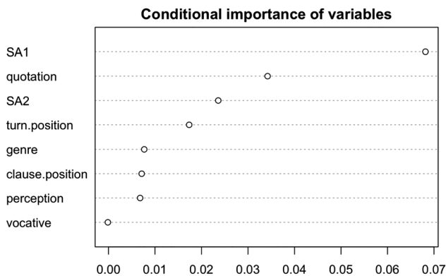
Figure 2: Random forest of the conditional importance of variables.
