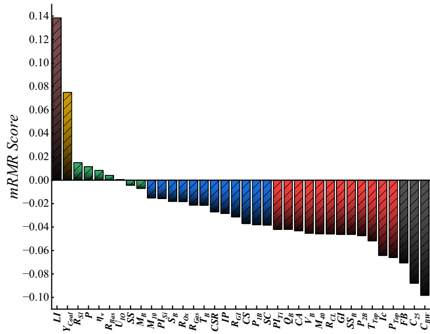
Figure S3: mRMR scores of the 36 features.
