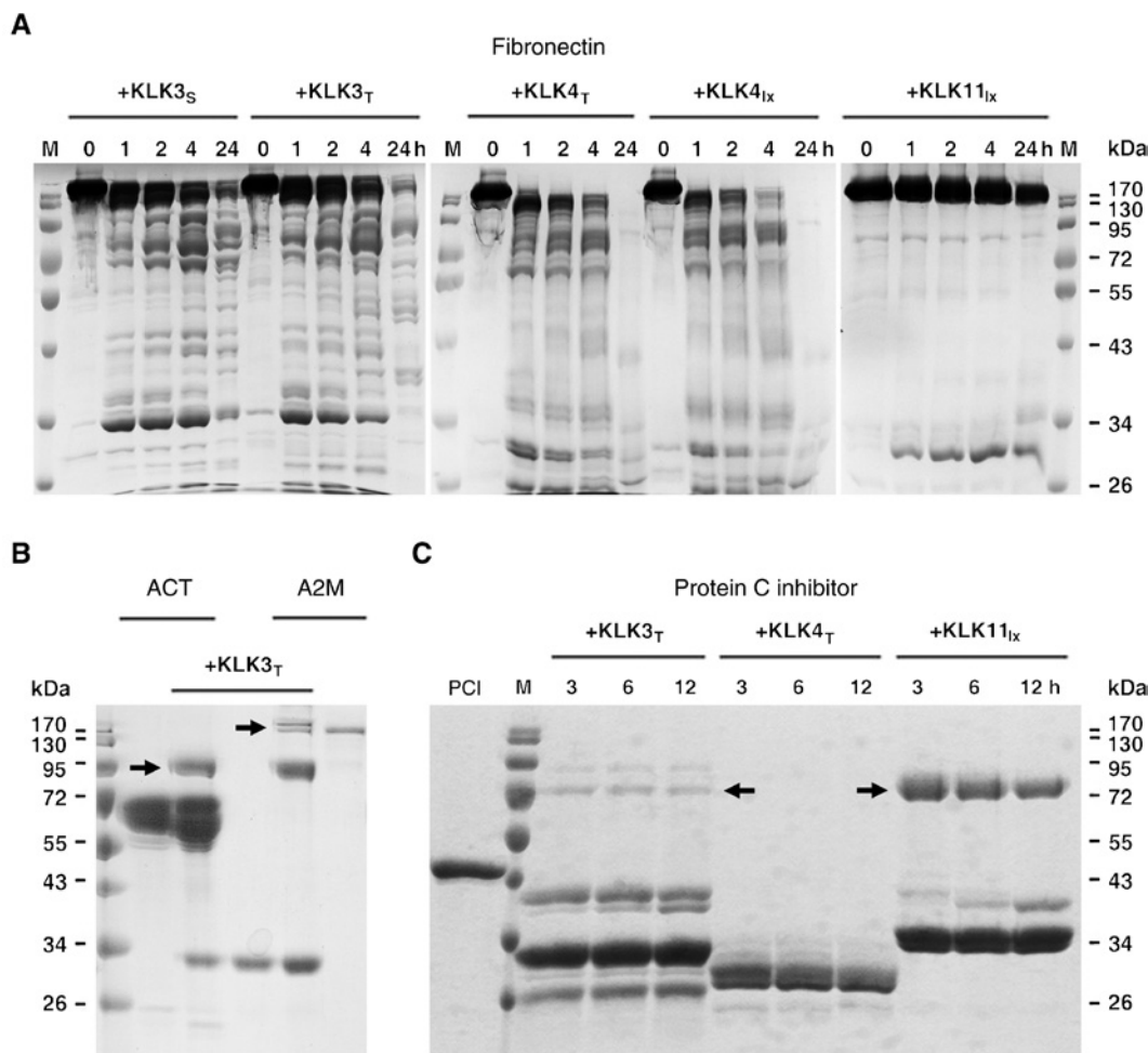
Figure 5: Turnover of fibronectin by various glycosylated KLKs 3, 4, and 11 and their interaction with physiological inhibitors.
