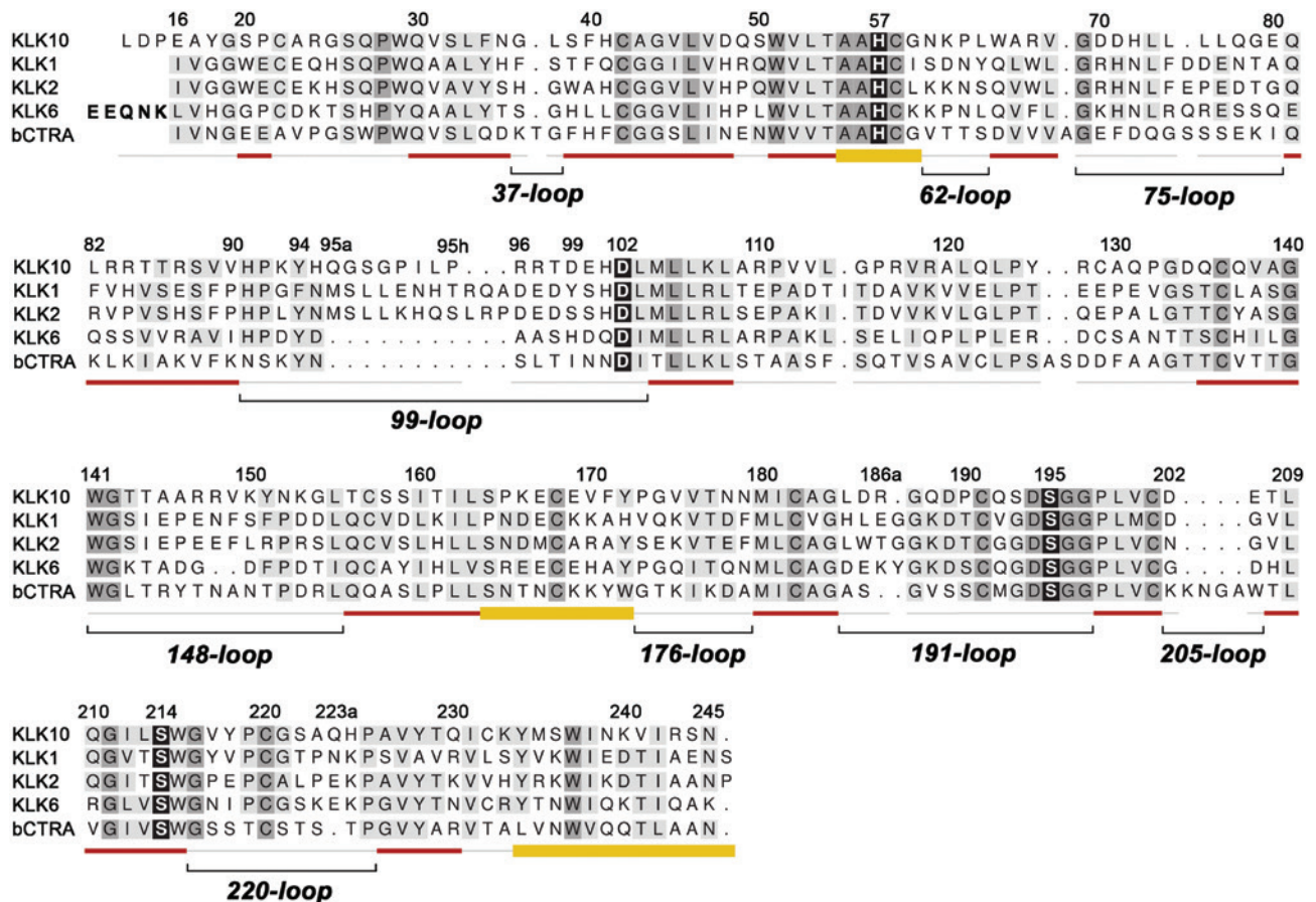
Figure 1: Structure-based alignment of KLK10 with KLKs 1, 2, 6 and bovine chymotrypsin (bCTRA) as numbering reference. The degree of conservation is indicated by darker background. The catalytic triad residues, and the 'fourth' triad residue Ser214 are shown with black background. Secondary structure is depicted as red strands and yellow helices. Loops are shown as light gray lines or, in the case of the relevant surface loops, with additional black lines and names according to the central residue numbering scheme. Insertions with respect to chymotrypsinogen as Gln95A are designated 95a with small letters. The propeptide of KLK6 is indicated with bold letters. Active KLK10 exhibits some uncommon features compared to the other trypsin-like serine proteases, such as Glu16 and the extended N-terminus starting with Leu13. Also the hydrophobic 75-loop segment with four Leu residues is unusual, as well as the 99-loop, which resembles the classical kallikrein loop of KLKs 1, 2 and 3 in length. Instead of a Ser, Thr or Ala, KLK10 possesses the unique Pro190, which may contribute to the mixed tryptic/hydrophobic substrate preference. Finally, Ser193 replaces the highly conserved Gly193 of the oxyanion hole and may considerably influence substrate binding and turnover.
