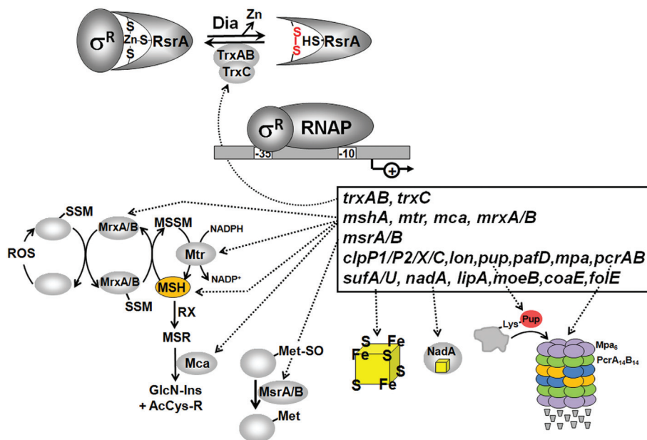
Figure 9: Redox regulation of the ZAS factor RsrA and its cognate sigma factor SigR in S. coelicolor and role of the SigR-regulon. RsrA is a redox-sensitive zinc-binding anti-sigma (ZAS) factor in S. coelicolor that sequesters its cognate sigma factor SigR under reducing conditions. Diamide stress leads to intramolecular disulfide formation in RsrA, resulting in Zn release and relief of SigR. Free SigR activates transcription of the SigR-regulon that functions to restore the thiol-redox balance. The SigR-regulon includes genes for thioredoxins and thioredoxin reductase ( trxAB , trxC ), enzymes for mycothiol biosynthesis and recycling ( mshA , mca , mtr ), mycoredoxins ( mrxA , mrxB ), methionine sulfoxide reductase ( msrA , msrB ), protein quality control machinery ( pepN , ssrA , clpP1P2 , clpX , clpC , lon ), ubiquitin-like protein-conjugation pathway and proteasomal components ( pup , mpa , pafD , prcAB ), Fe-S assembly components ( sufA , sufU ) and Fe-S containing enzymes ( nadA , lipA ), biosynthesis enzymes for the cofactors Fe-S, folate, CoASH and lipoic acid ( moeB , coaE , folE , lipA ). Examples for SigR-regulon genes and their functions are also listed in Table 6.
