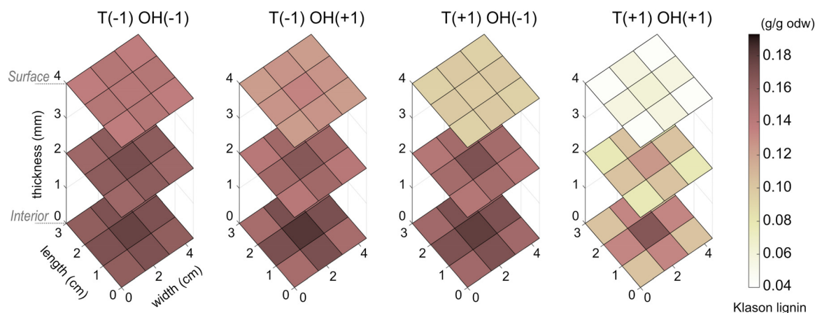
Figure 7: Distribution of Klason lignin (g/g of dry wood) in the nine sections of wood chips after 45 min of batch kraft cooking. Cooking conditions from left to right: 145 °C & 0.25 mol \text{HO}^- /kg liq., 145 °C & 0.55 mol \text{HO}^- /kg liq., 165 °C & 0.25 mol \text{HO}^- /kg liq., 165 °C & 0.55 mol \text{HO}^- /kg liq. Estimated error = 5 % (refer to Supplementary Material).
