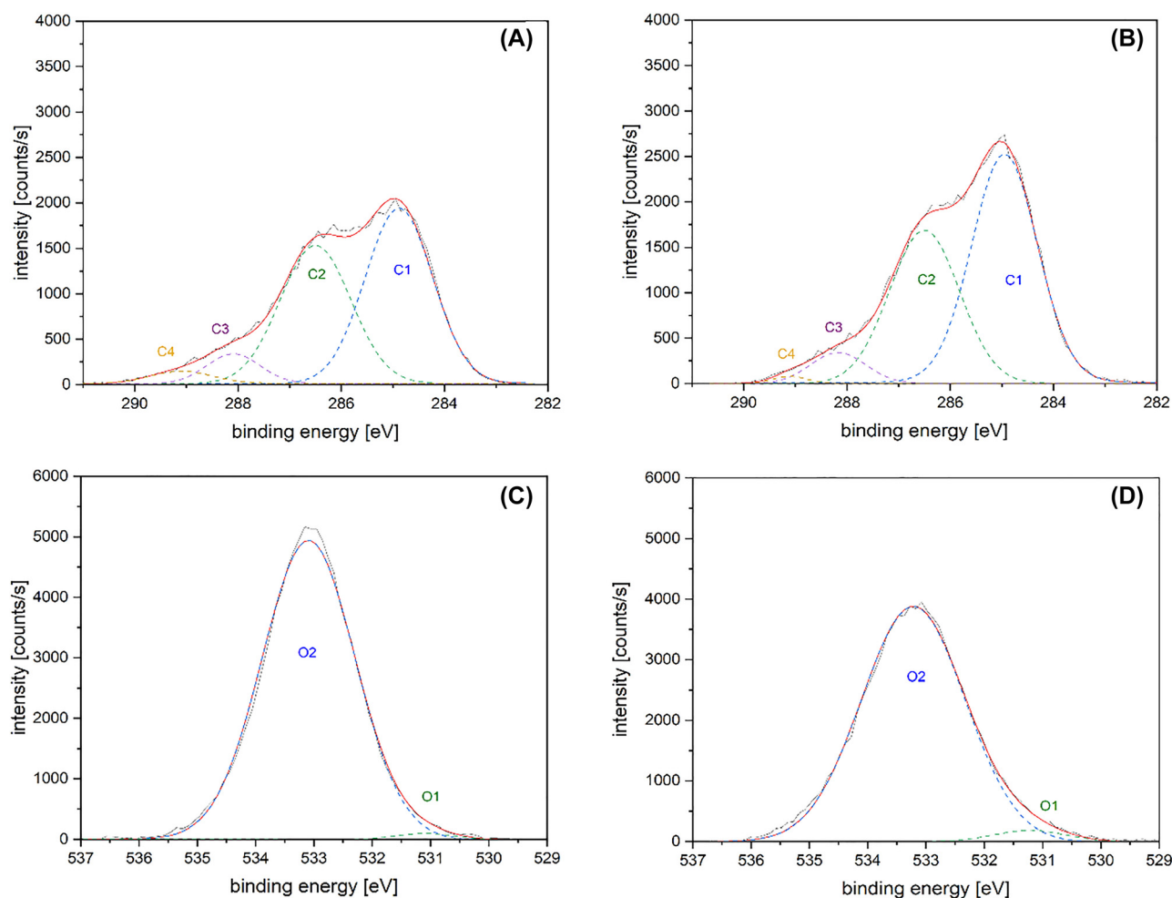
Figure 2: High-resolution spectra of the C1s and O1s energy levels of recently-cut (A, C) and archaeological samples (B, D) of oak.
