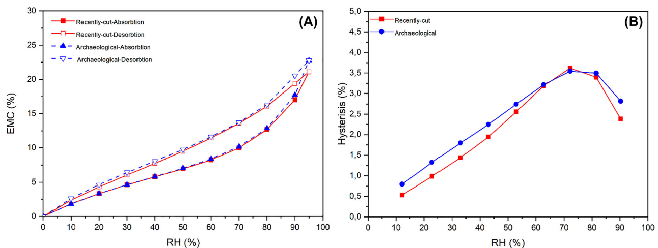
Figure 4: Adsorption and desorption isotherms (A) and sorption hysteresis (B) of recently-cut and archaeological oak at changing RH levels.
