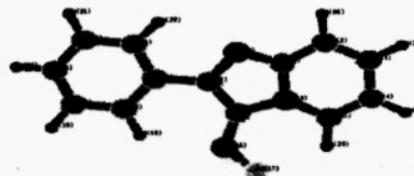
Fig. 2 Most stable conformation obtained for 2-phenyl-3-
