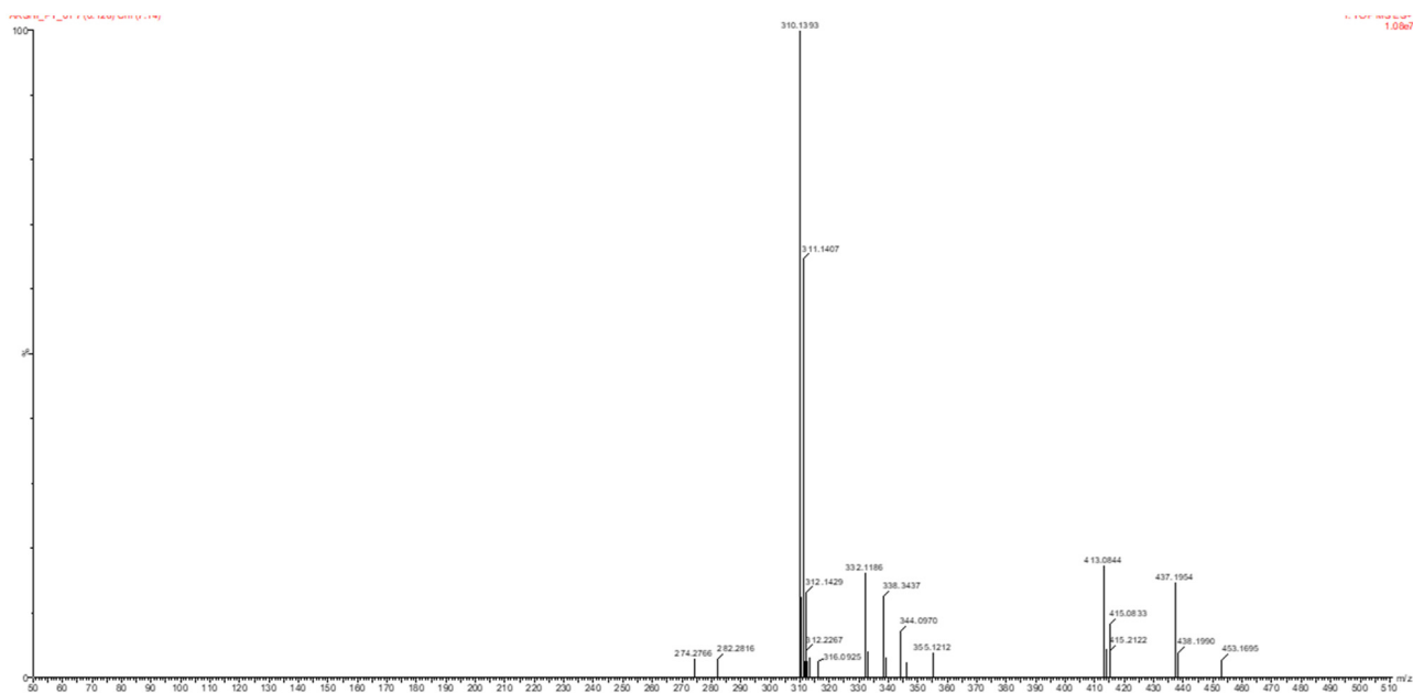
Figure S22: LCMS-HRMS spectra of compound 2a.
