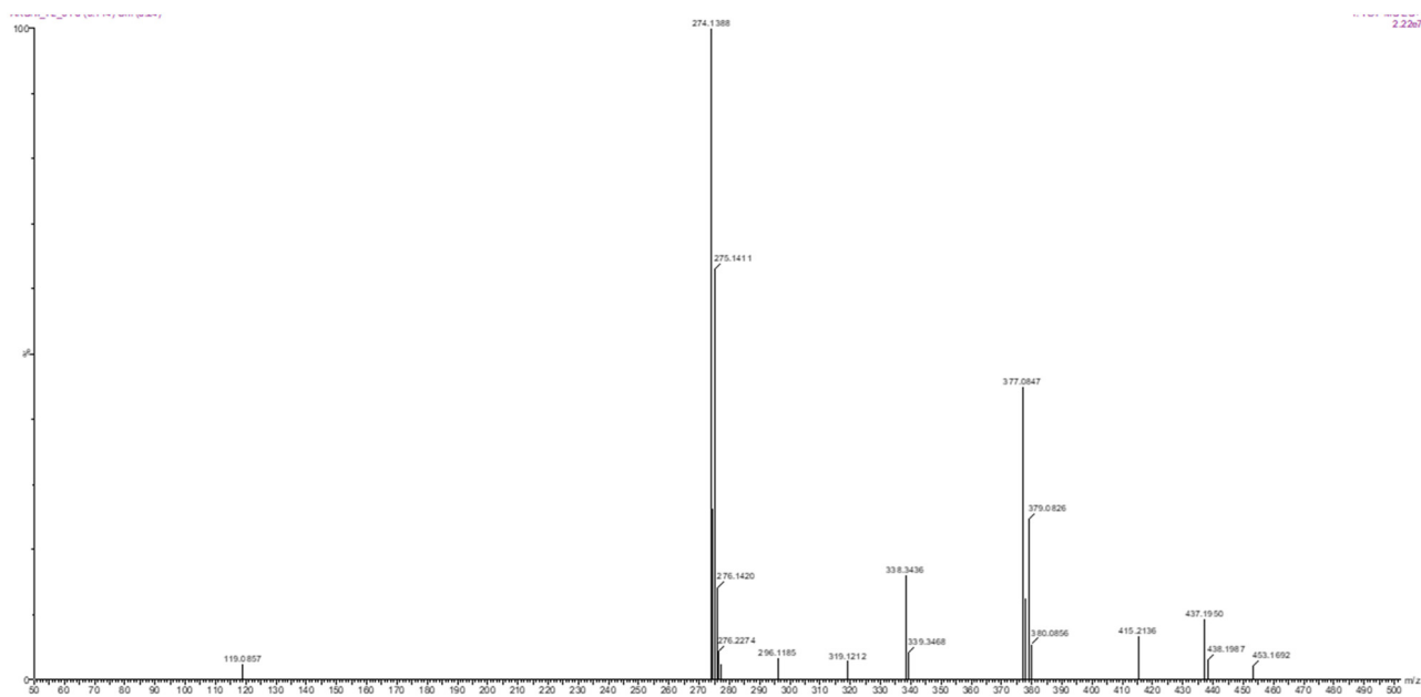
Figure S25: LCMS-HRMS spectra of compound 3a.
