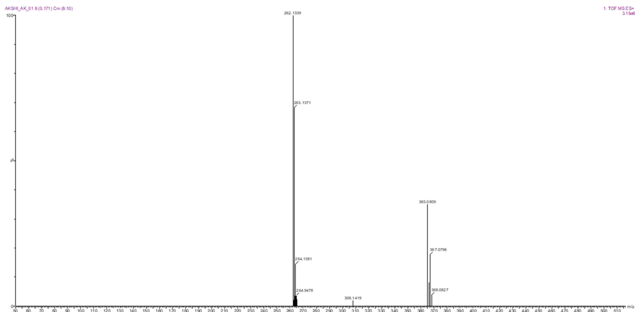
Figure S19: LCMS-HRMS spectra of compound 1a.
