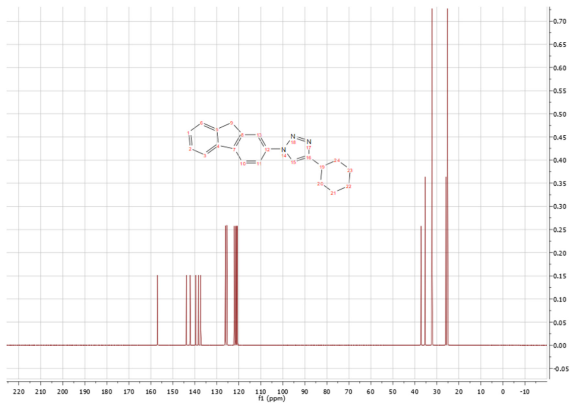
Figure S18: ^{13}\text{C} -spectra of compound 3c.
