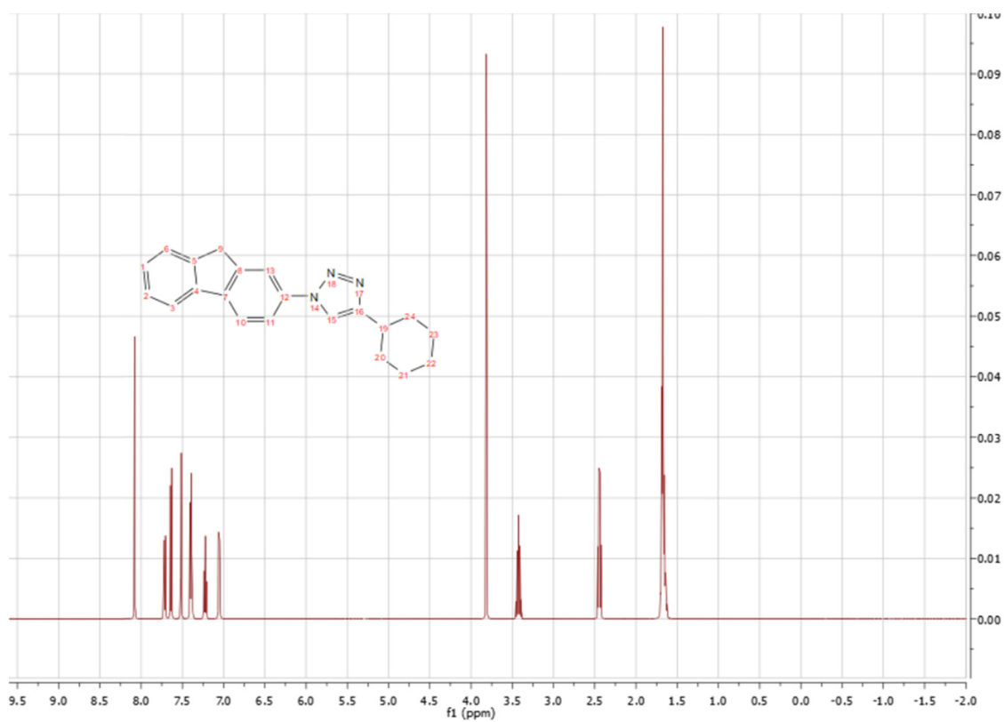
Figure S17: 1 H-spectra of compound 3c.
