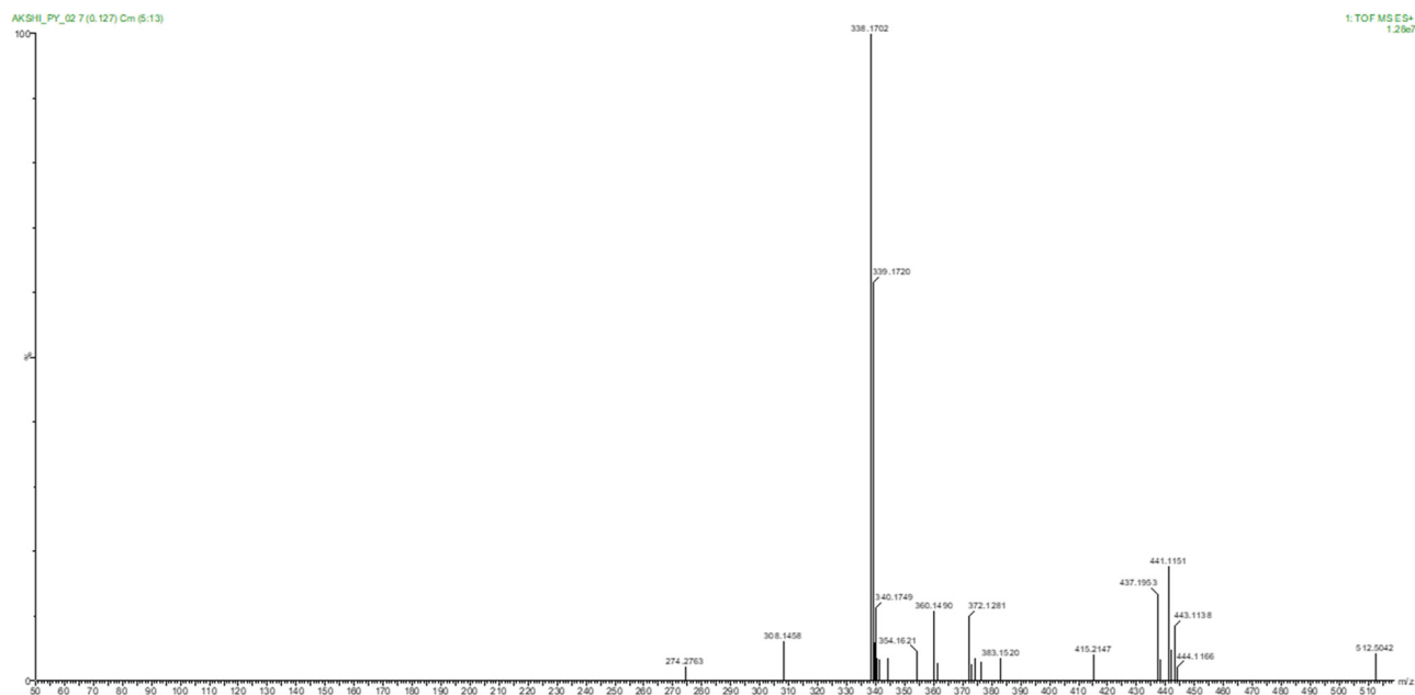
Figure S23: LCMS-HRMS spectra of compound 2b.
