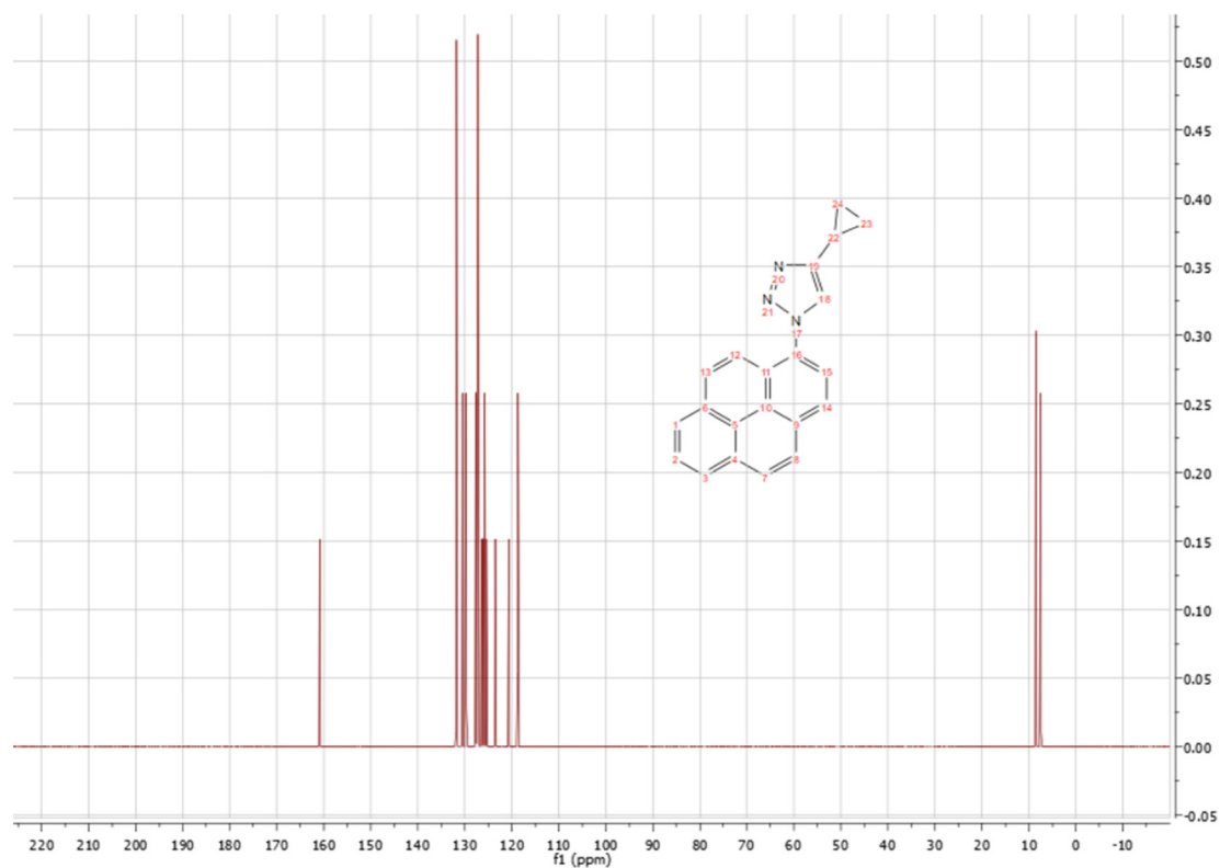
Figure S8: 13 C-spectra of compound 2a.
