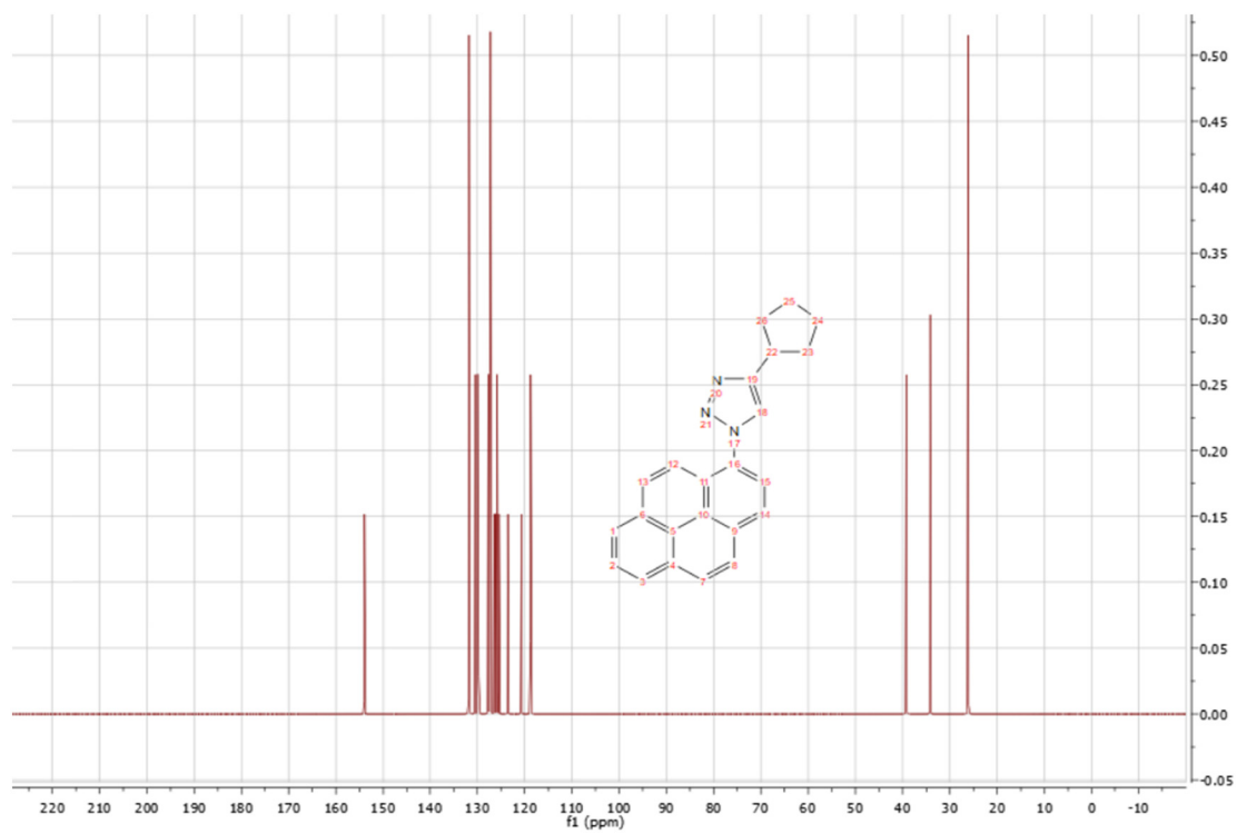
Figure S10: ^{13}\text{C} -spectra of compound 2b.
