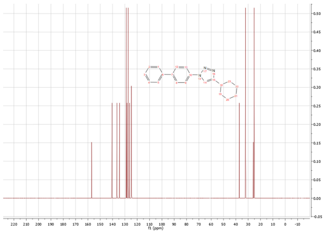
Figure S6: 13 C-spectra of compound 1c.
