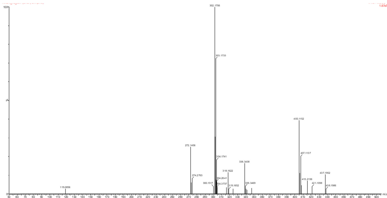
Figure S26: LCMS-HRMS spectra of compound 3b.
