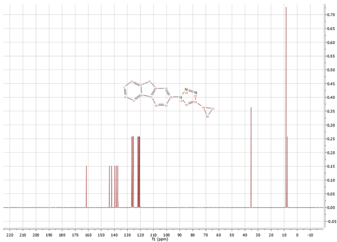
Figure S14: 13 C-spectra of compound 3a.
