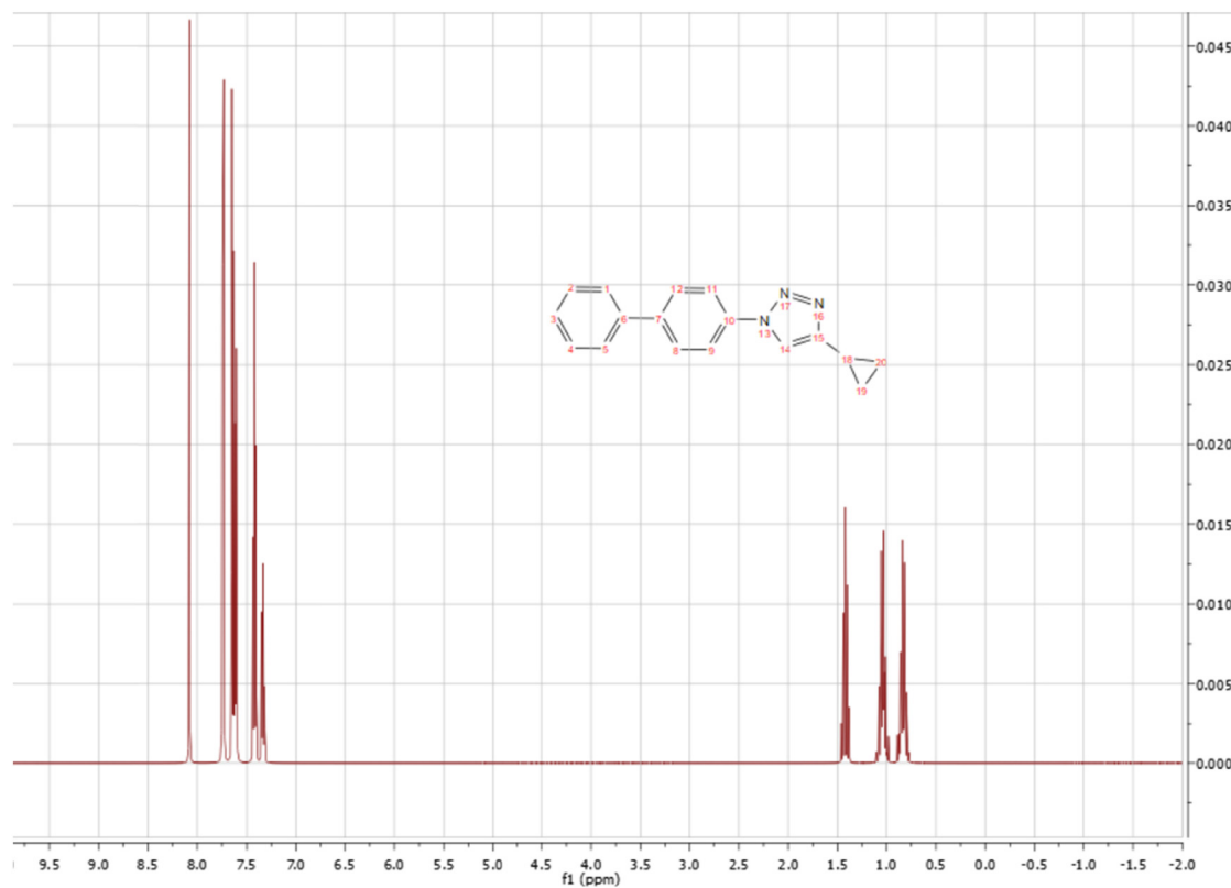
Figure S1: ^1\text{H} -spectra of compound 1a.
