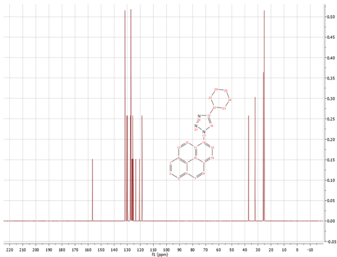
Figure S12: ^{13}\text{C} -spectra of compound 2c.
