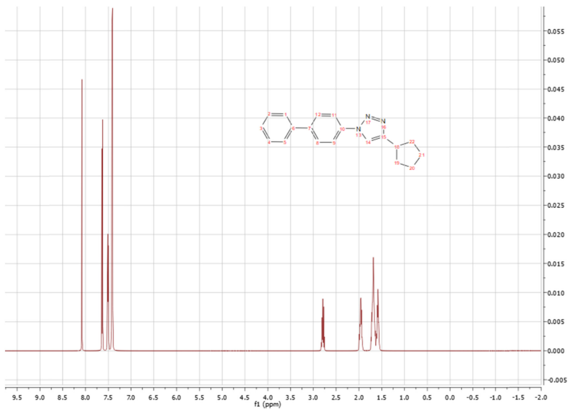
Figure S3: ^1\text{H} -spectra of compound 1b.
