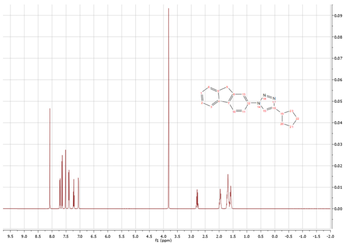
Figure S15: 1 H-spectra of compound 3b.
