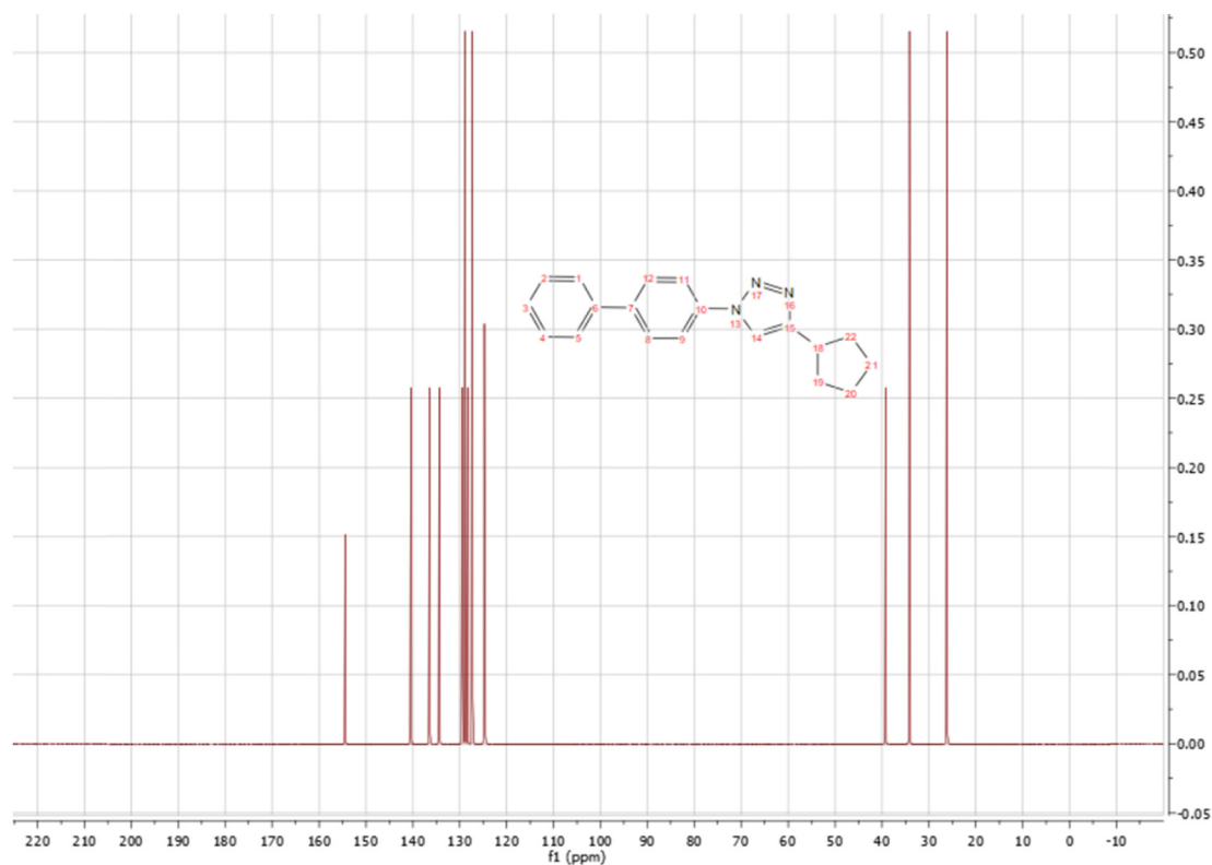
Figure S4: ^{13}\text{C} -spectra of compound 1b.
