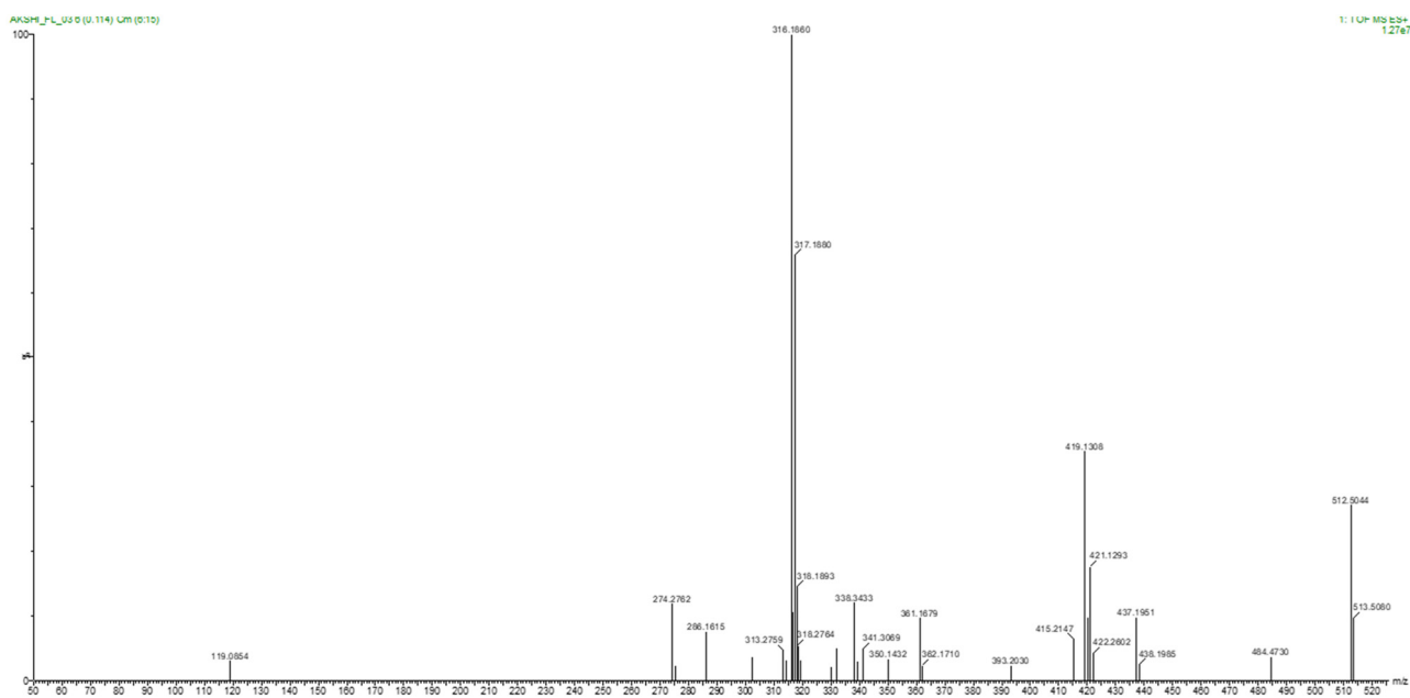
Figure S27: LCMS-HRMS spectra of compound 3c.
