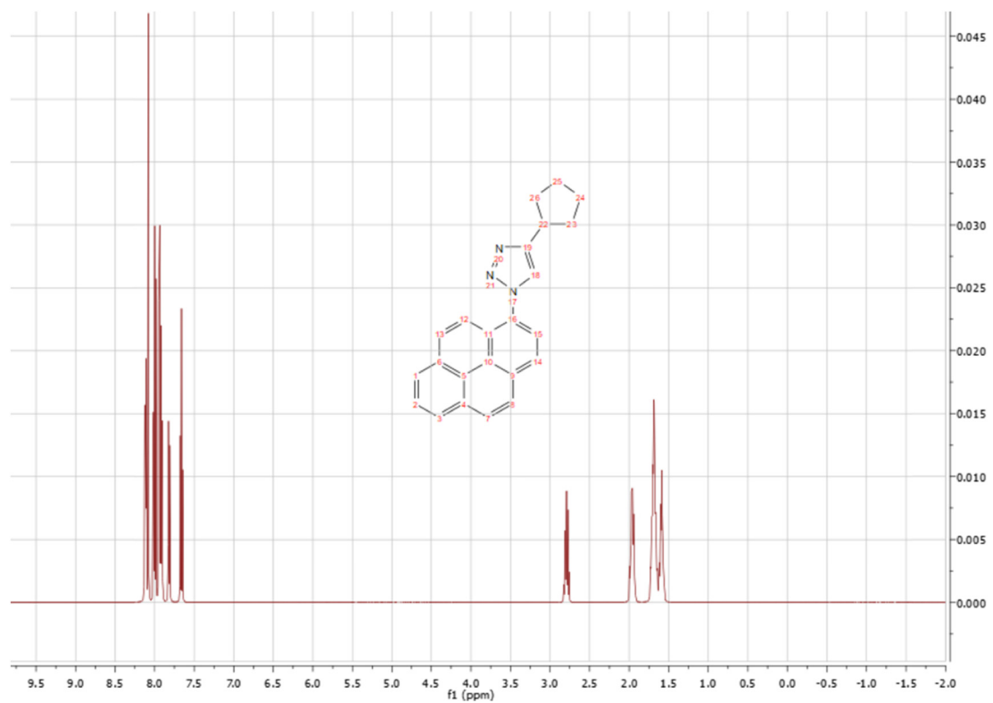
Figure S9: 1 H-spectra of compound 2b.
