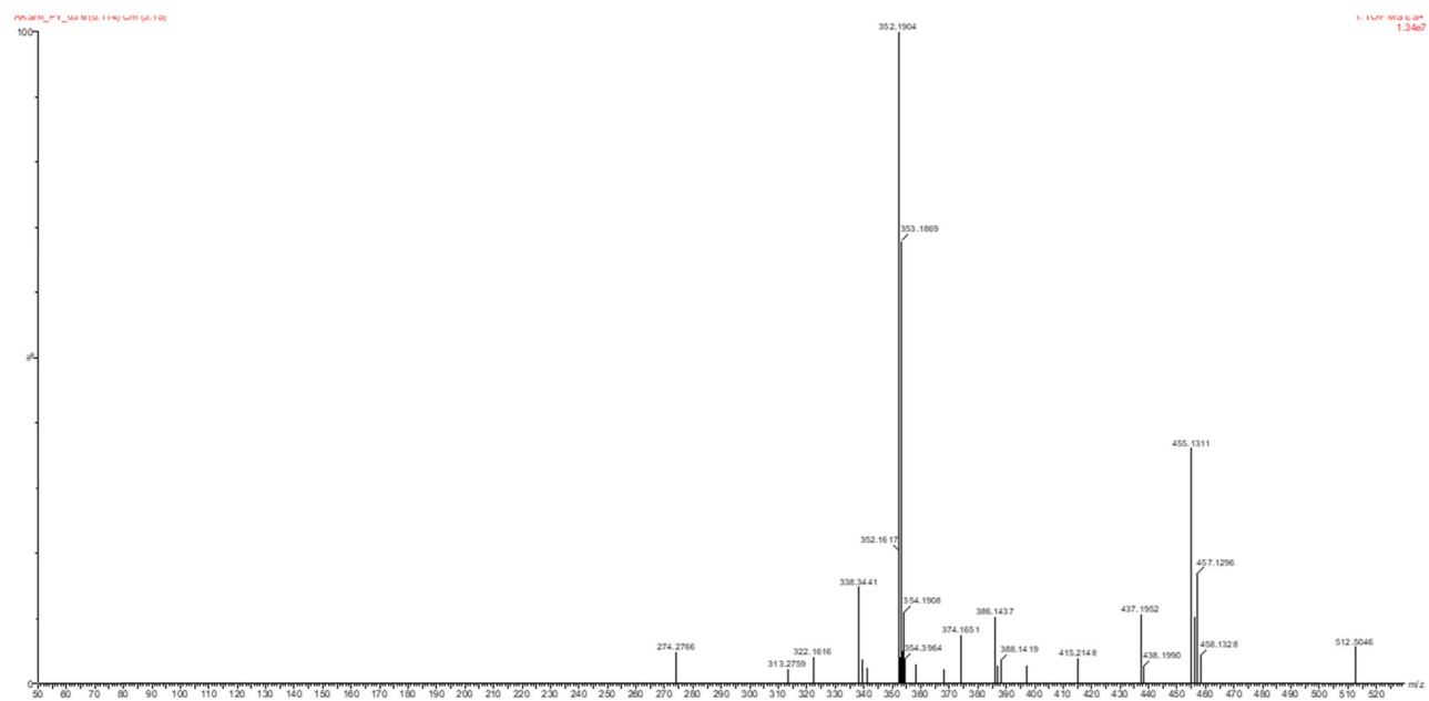
Figure S24: LCMS-HRMS spectra of compound 2c.
