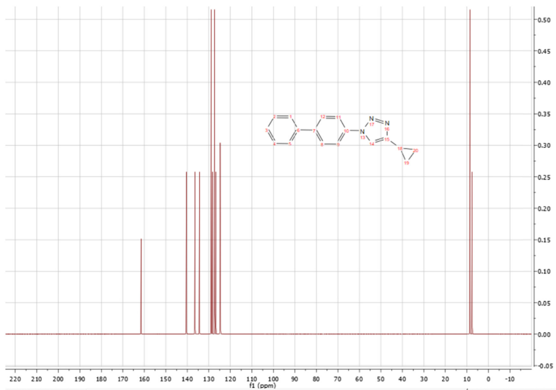
Figure S2: ^{13}\text{C} -spectra of compound 1a.
