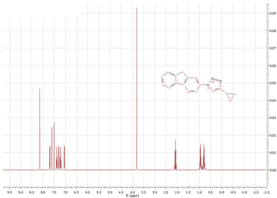
Figure S13: ^1\text{H} -spectra of compound 3a.
