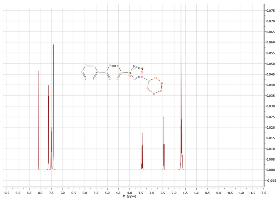
Figure S5: ^1\text{H} -spectra of compound 1c.
