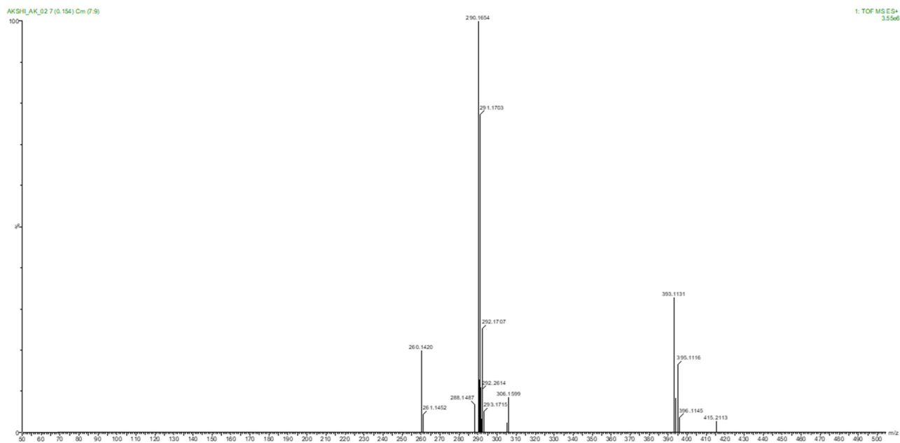
Figure S20: LCMS-HRMS spectra of compound 1b.
