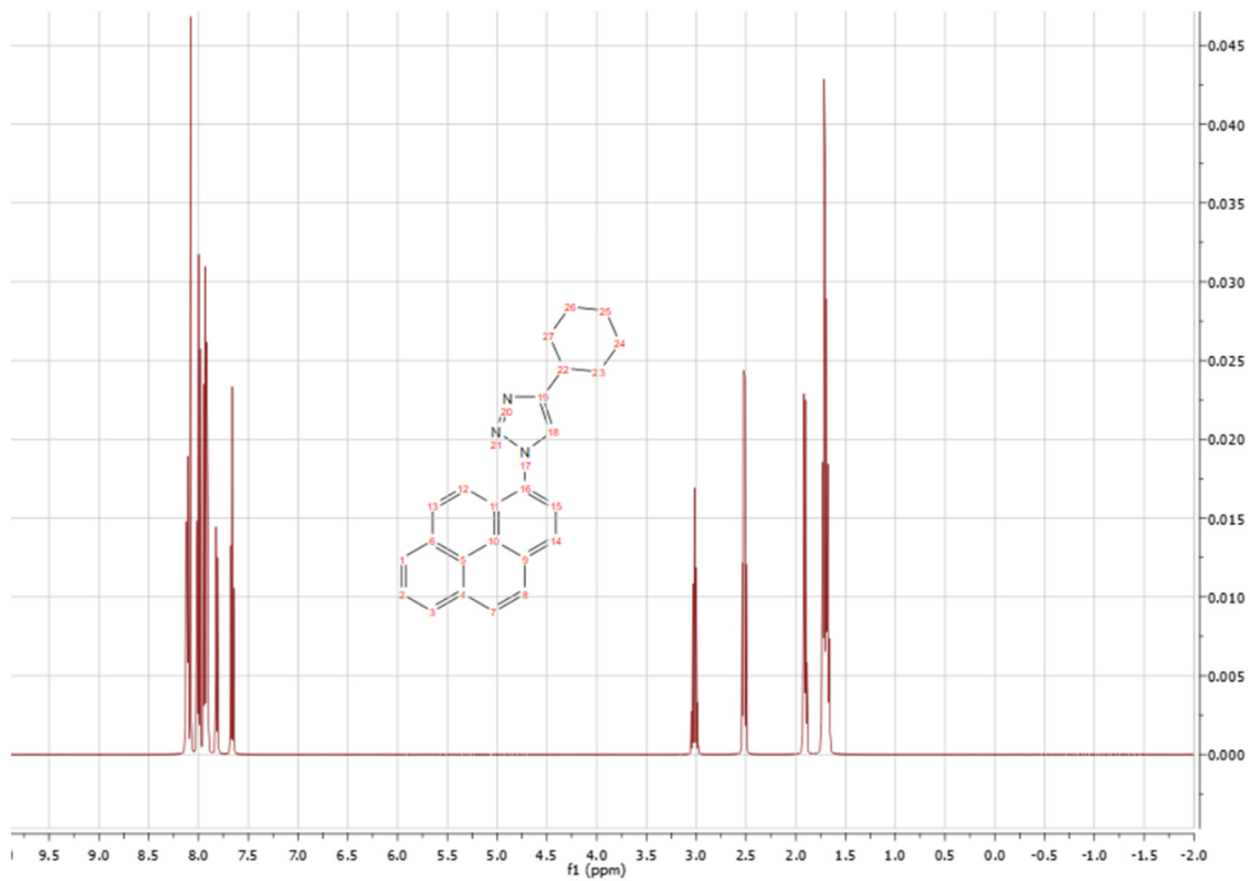
Figure S11: ^1\text{H} -spectra of compound 2c.
