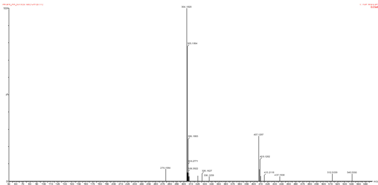
Figure S21: LCMS-HRMS spectra of compound 1c.
