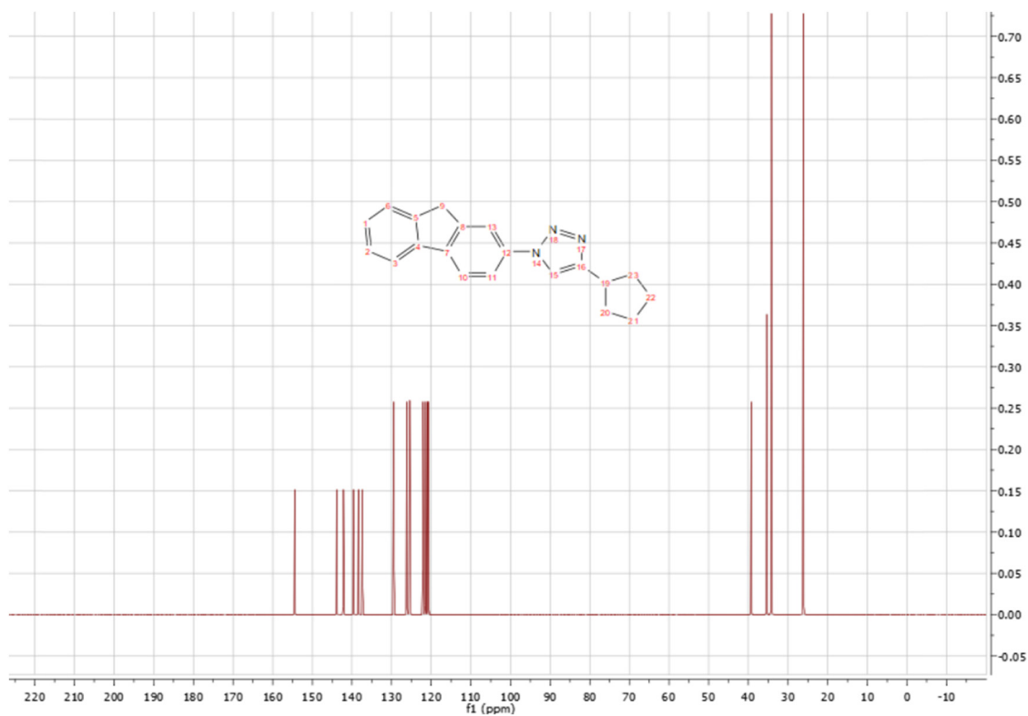
Figure S16: 13 C-spectra of compound 3b.
