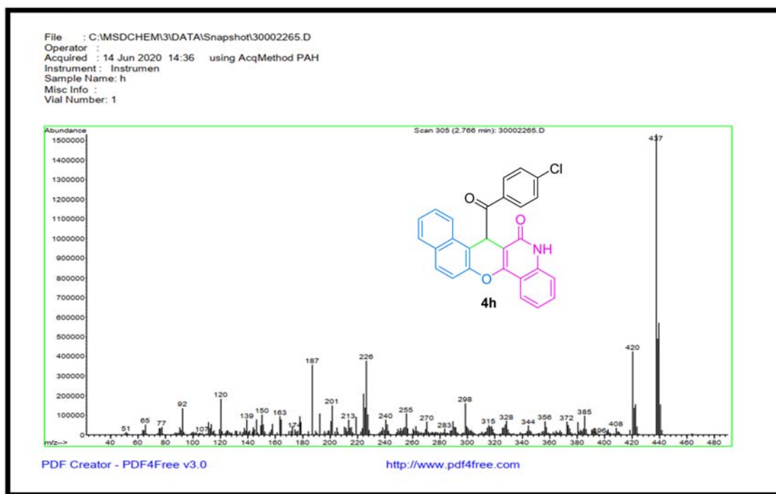
Figure S31: Mass spectrum of compound 4h.
