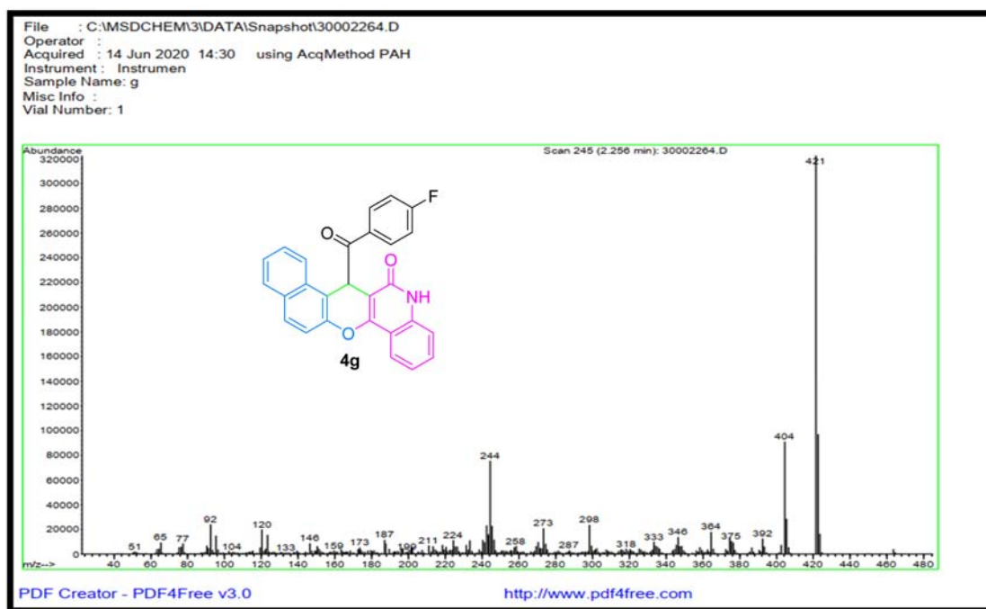
Figure S27: Mass spectrum of compound 4g .
