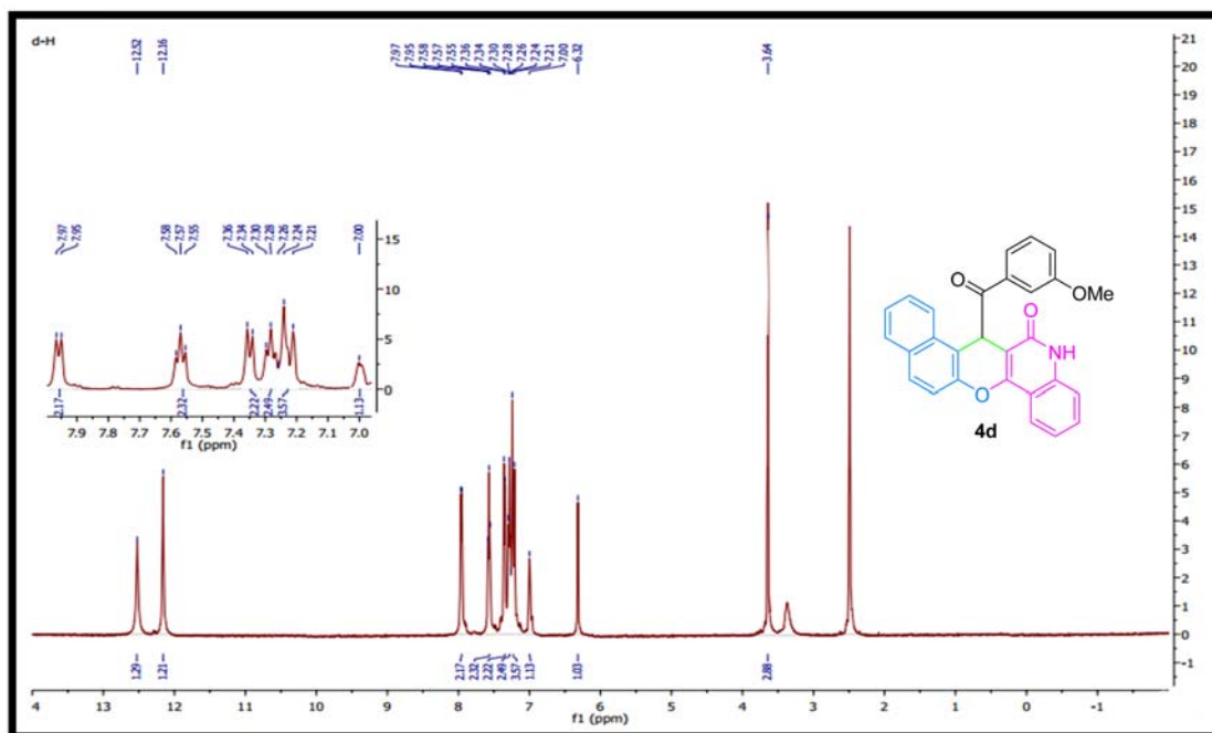
Figure S13: 1 H NMR spectrum of compound 4d.
