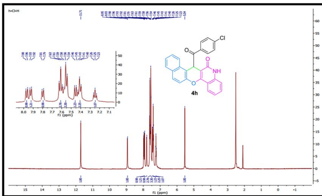
Figure S29: 1 H NMR spectrum of compound 4h .
