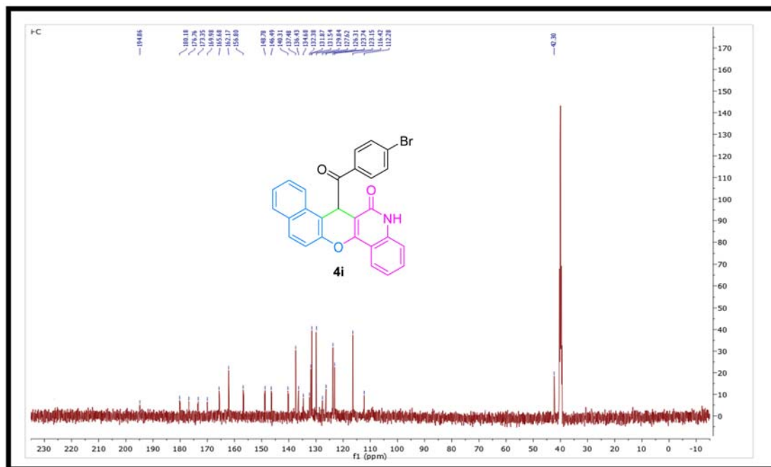
Figure S34: ^{13}\text{C} NMR spectrum of compound 4i .
