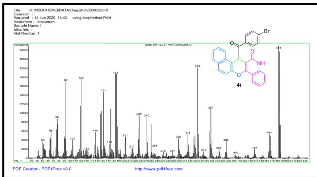
Figure S35: Mass spectrum of compound 4i .
