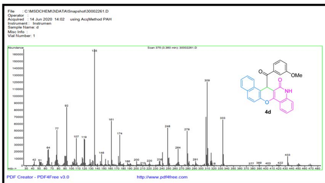
Figure S15: Mass spectrum of compound 4d.
