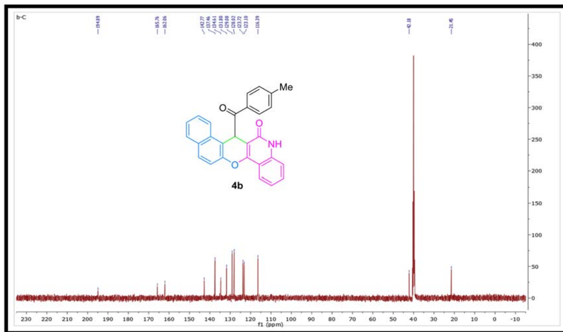
Figure S6: ^{13}\text{C} NMR spectrum of compound 4b .
