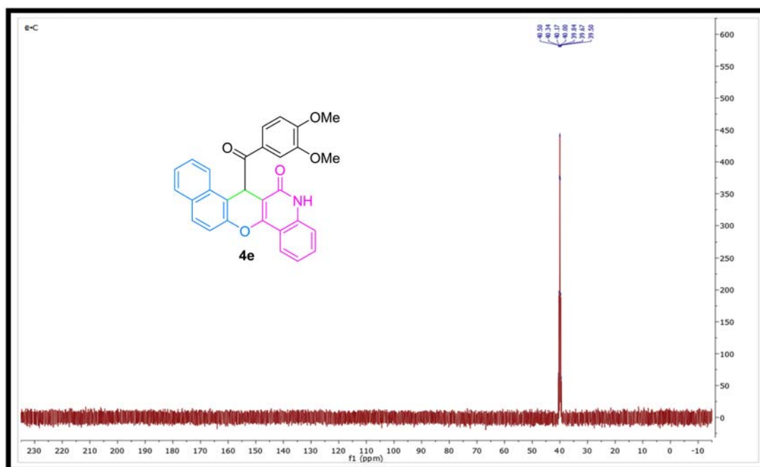
Figure S18: ^{13}\text{C} NMR spectrum of compound 4e .
