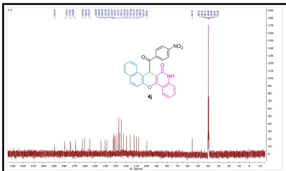
Figure S38: ^{13}\text{C} NMR spectrum of compound 4j .
