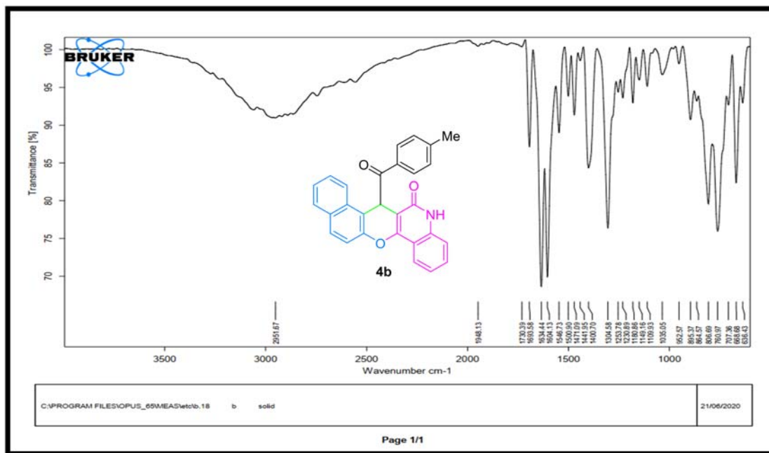
Figure S8: IR spectrum of compound 4b.
