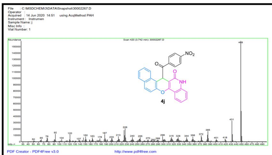
Figure S39: Mass spectrum of compound 4j .
