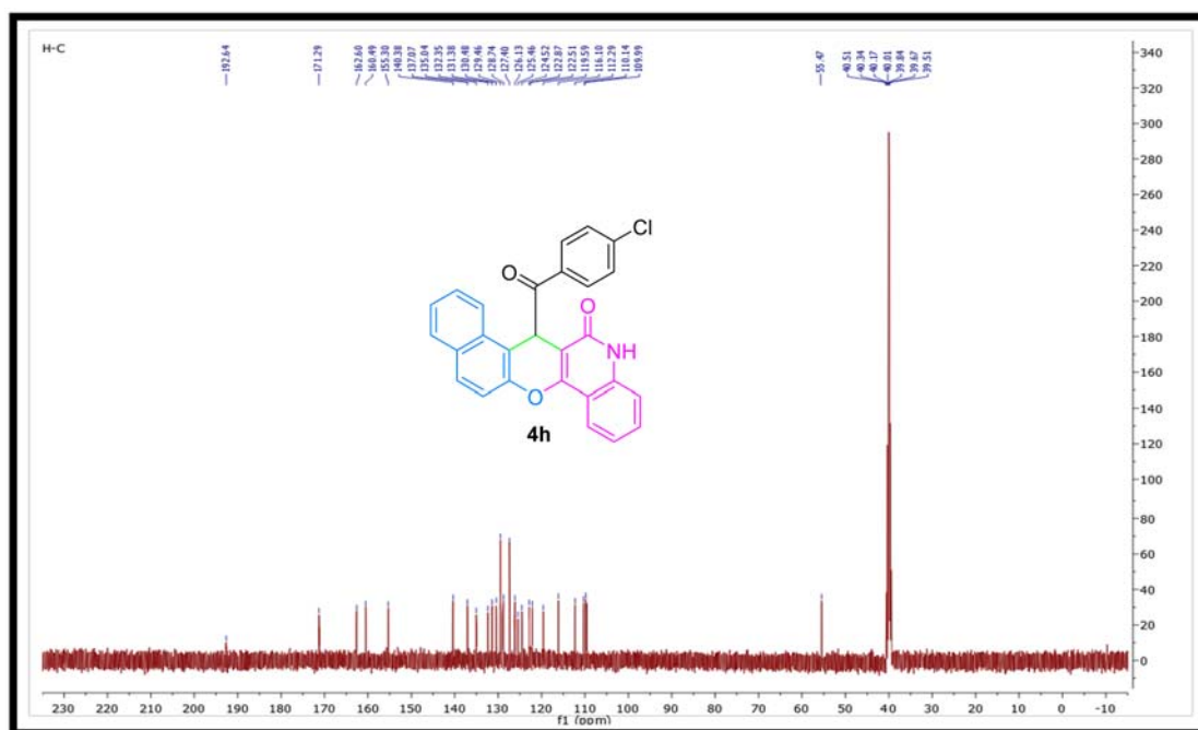
Figure S30: ^{13}\text{C} NMR spectrum of compound 4h.
