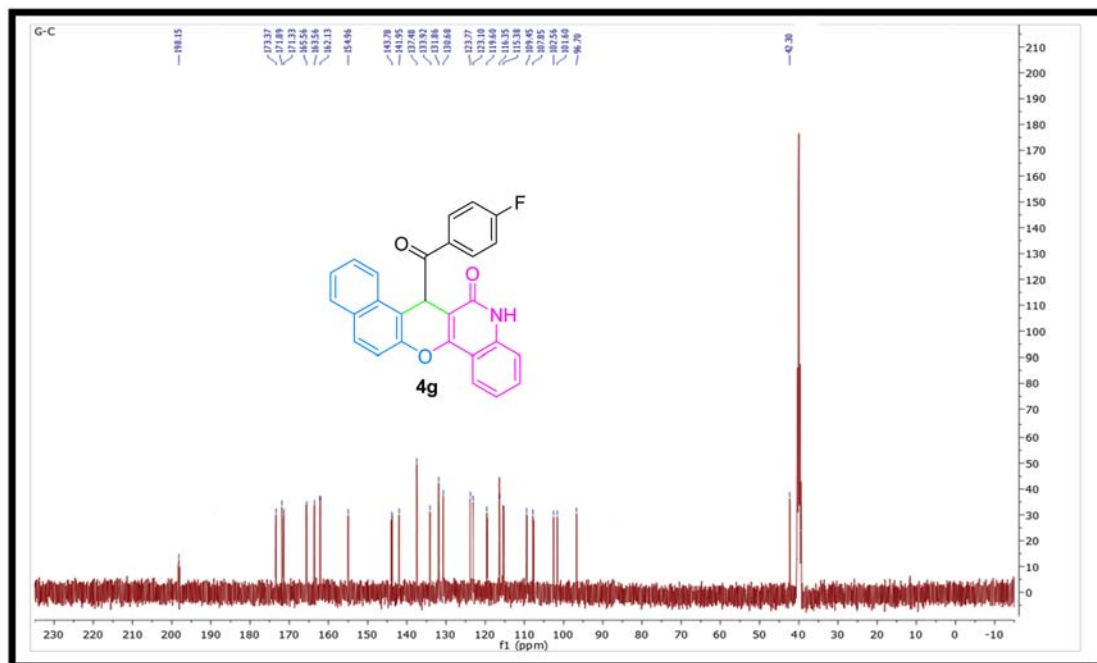
Figure S26: ^{13}\text{C} NMR spectrum of compound 4g .
