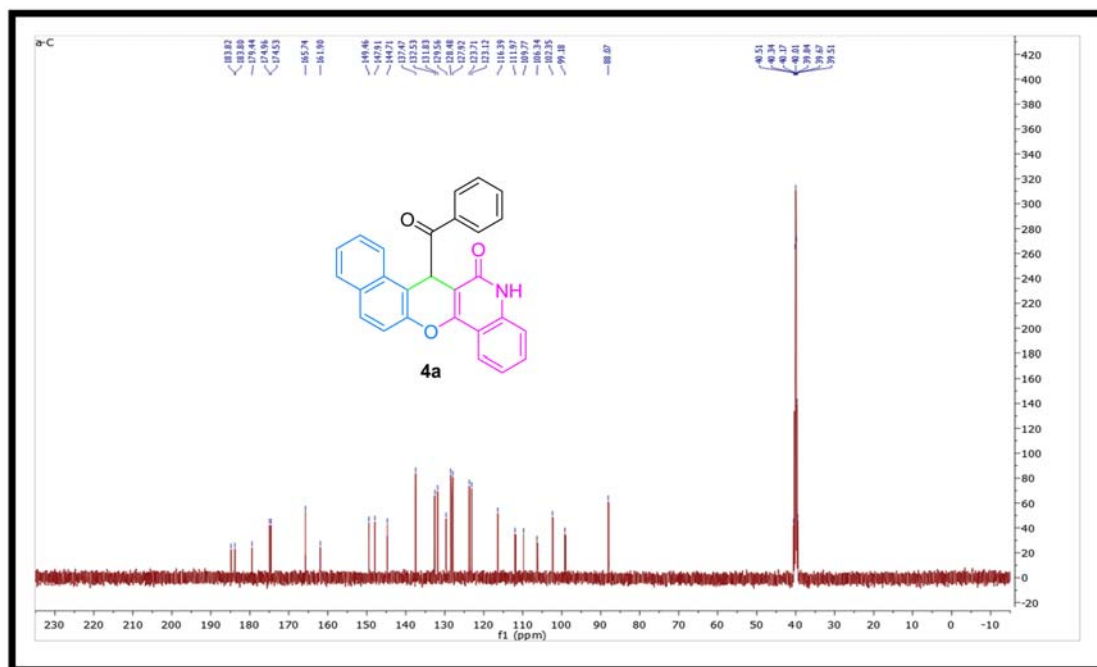
Figure S2: ^{13}\text{C} NMR spectrum of compound 4a.
