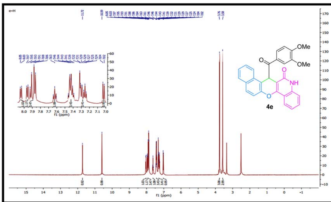
Figure S17: 1 H NMR spectrum of compound 4e.
