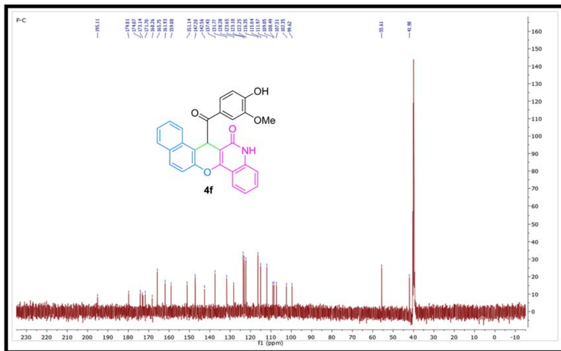
Figure S22: ^{13}\text{C} NMR spectrum of compound 4f .
