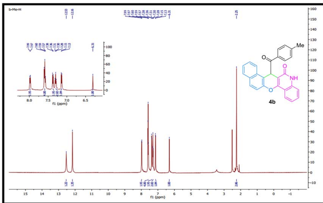
Figure S5: 1 H NMR spectrum of compound 4b.
