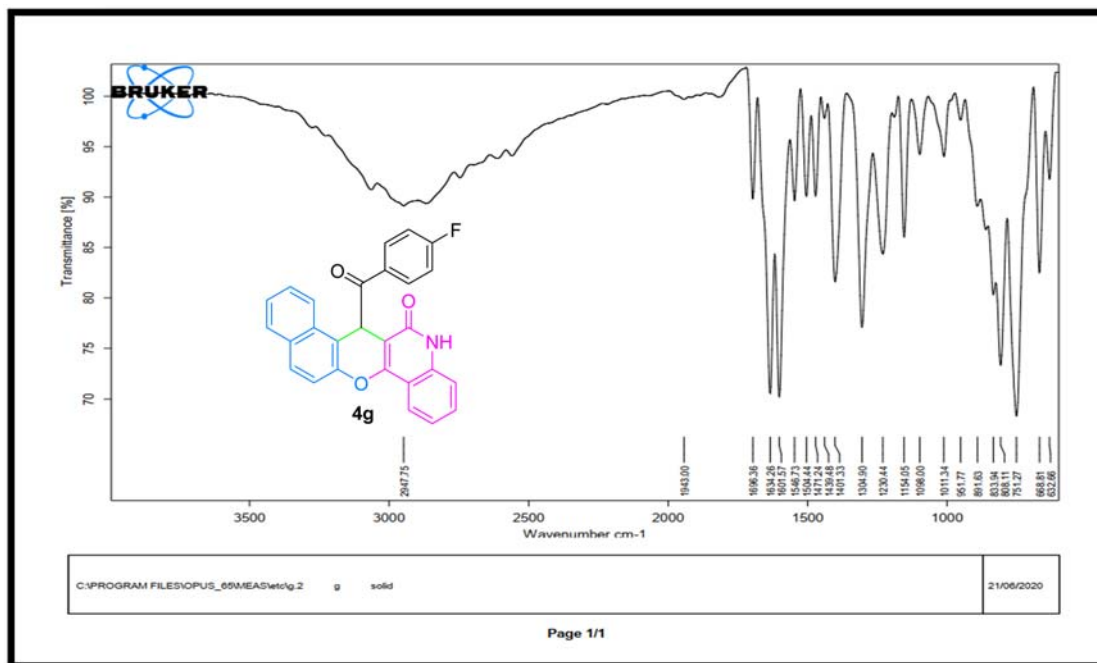
Figure S28: IR spectrum of compound 4g .
