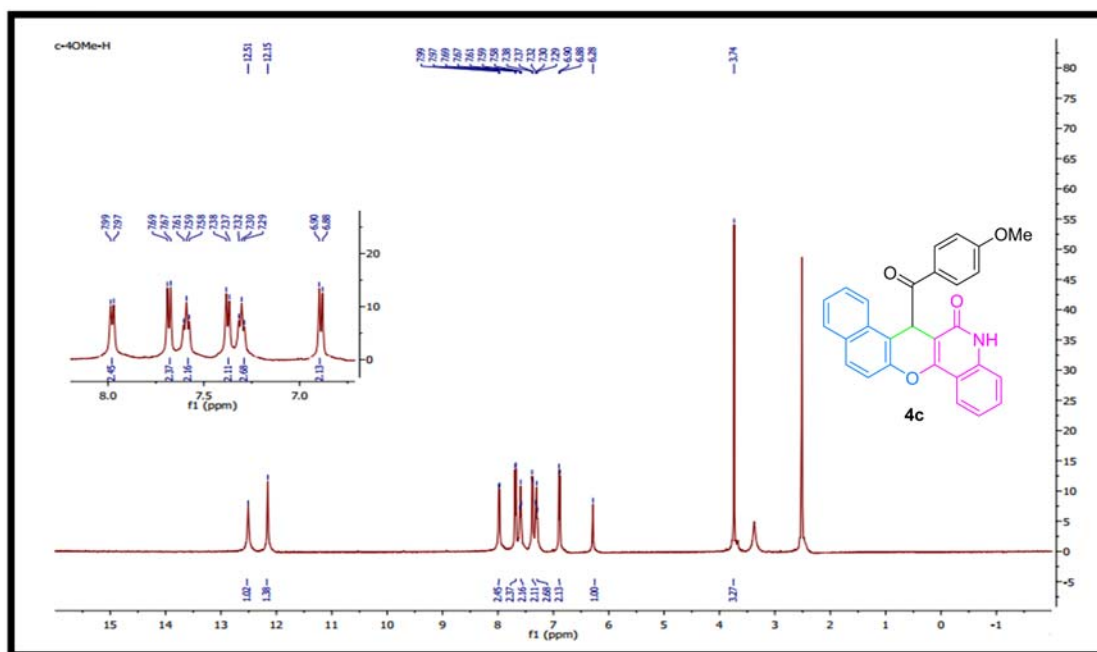
Figure S9: 1 H NMR spectrum of compound 4c.
