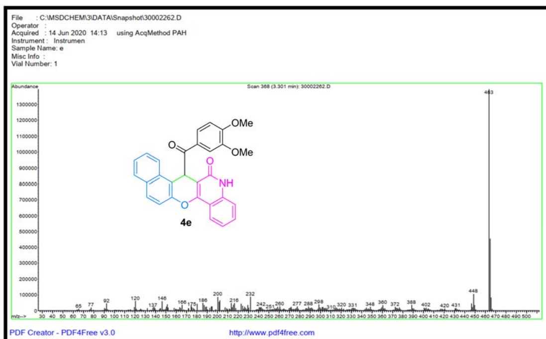
Figure S19: Mass spectrum of compound 4e .
