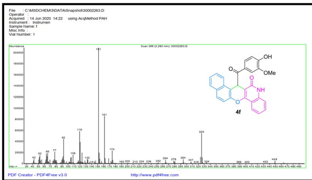
Figure S23: Mass spectrum of compound 4f .
