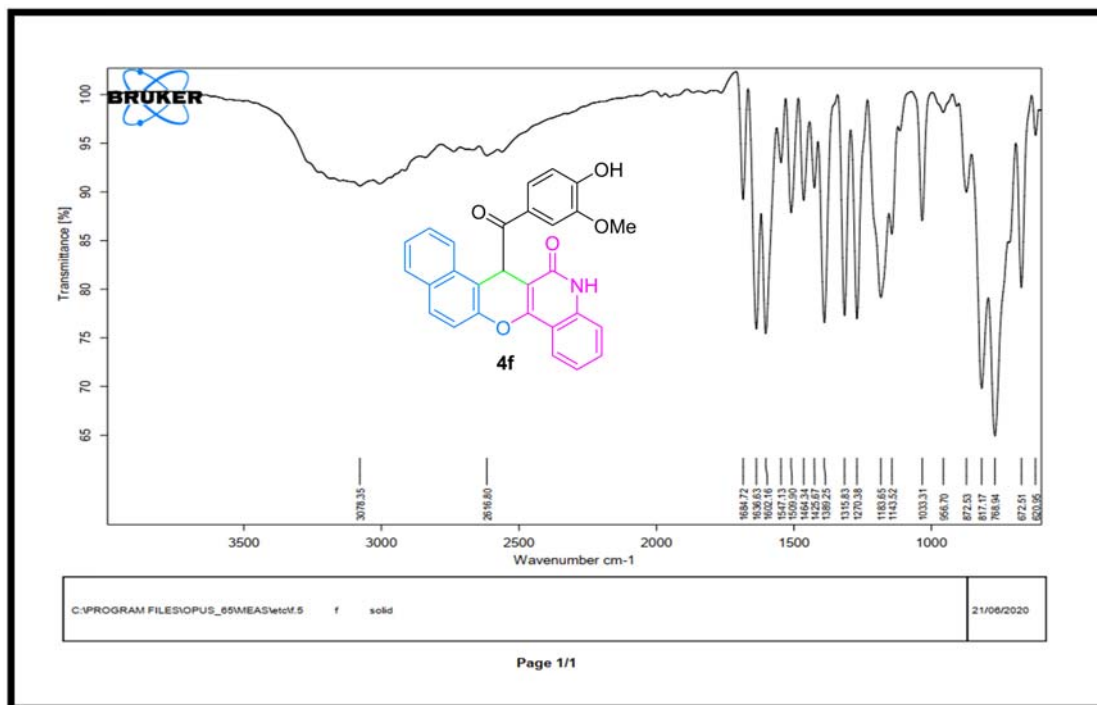
Figure S24: IR spectrum of compound 4f.
