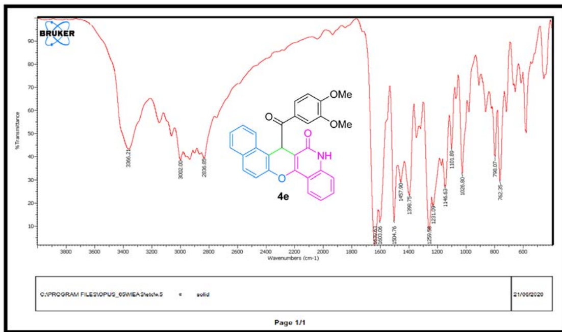
Figure S20: IR spectrum of compound 4e.
