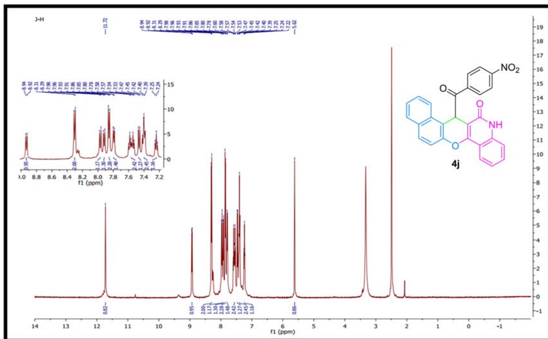
Figure S37: 1 H NMR spectrum of compound 4j.
