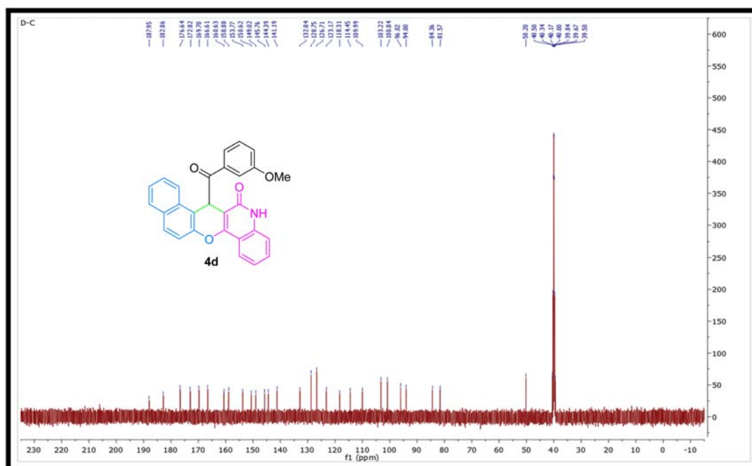
Figure S14: 13 C NMR spectrum of compound 4d.
