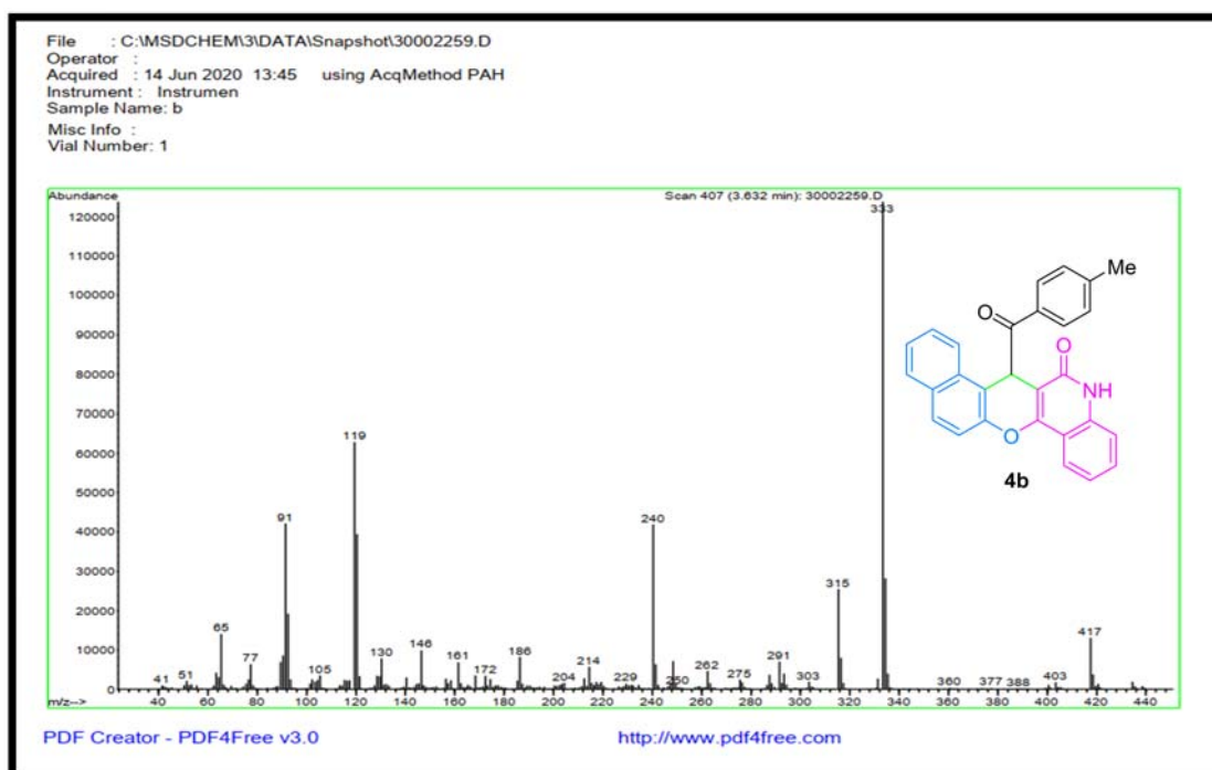
Figure S7: Mass spectrum of compound 4b .
