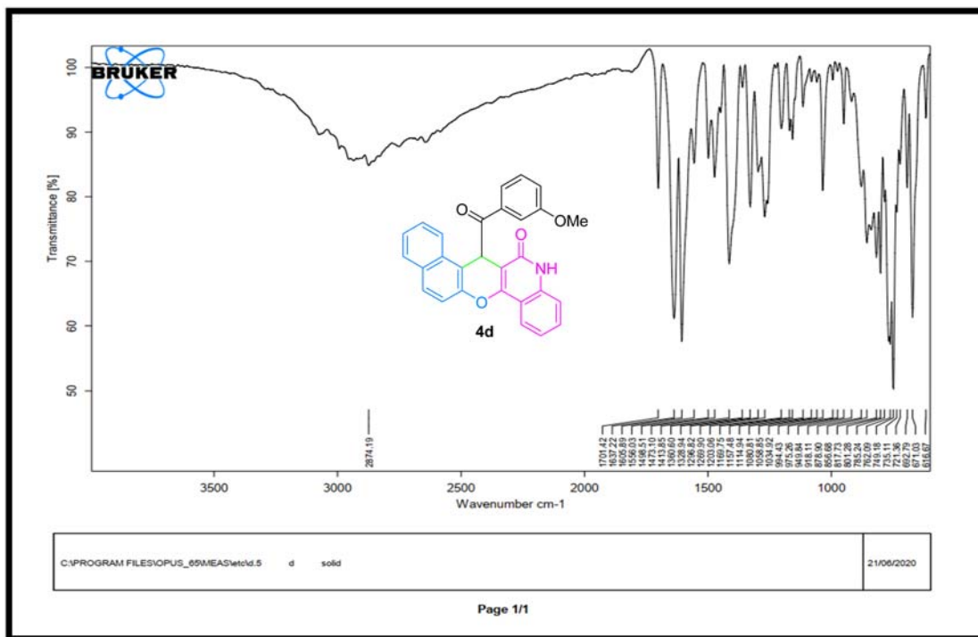
Figure S16: IR spectrum of compound 4d.
