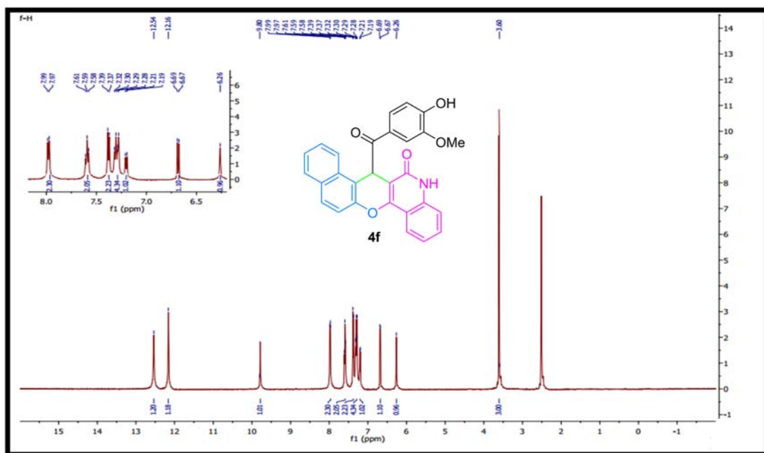
Figure S21: 1 H NMR spectrum of compound 4f.
