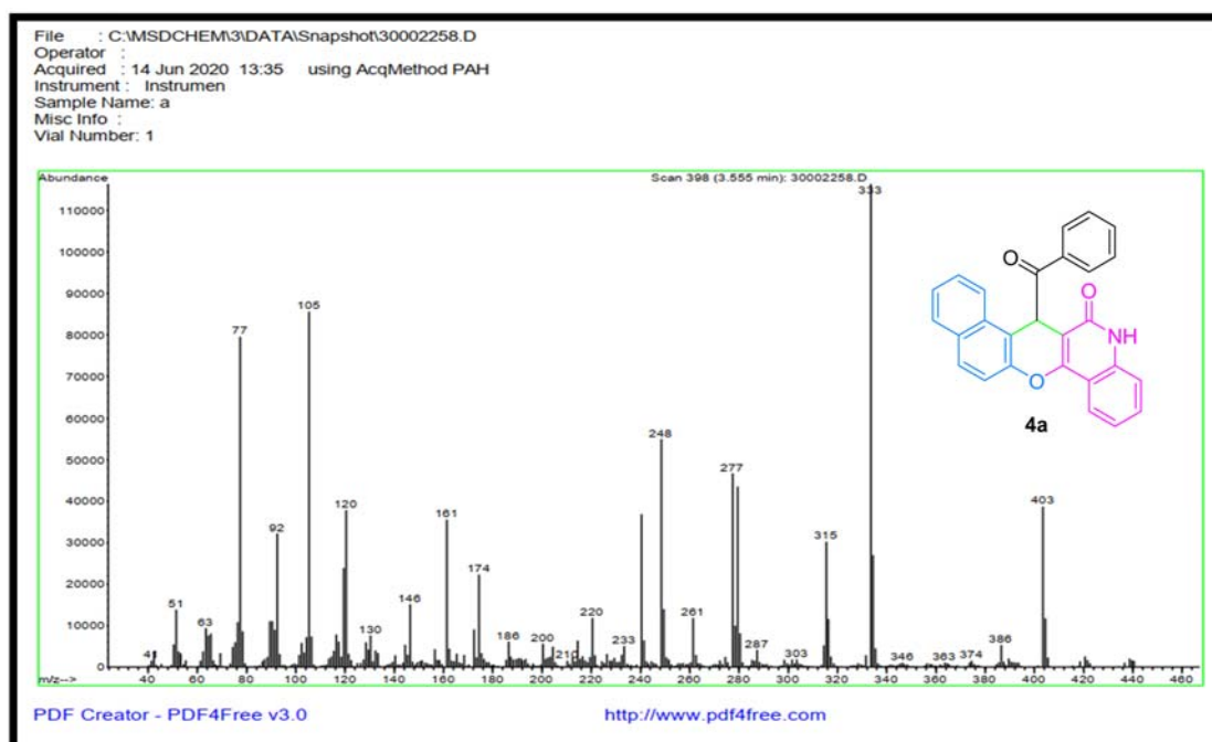
Figure S3: Mass spectrum of compound 4a.
