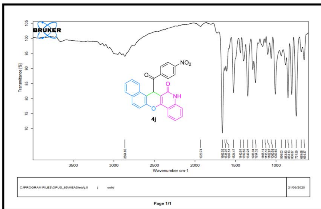
Figure S40: IR spectrum of compound 4j.
