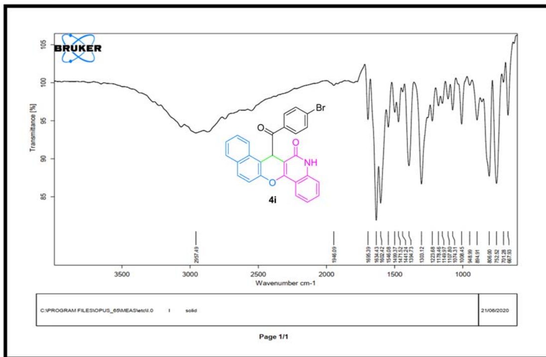
Figure S36: IR spectrum of compound 4i.
