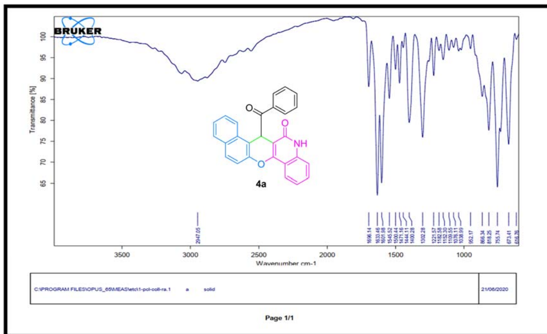
Figure S4: IR spectrum of compound 4a.
