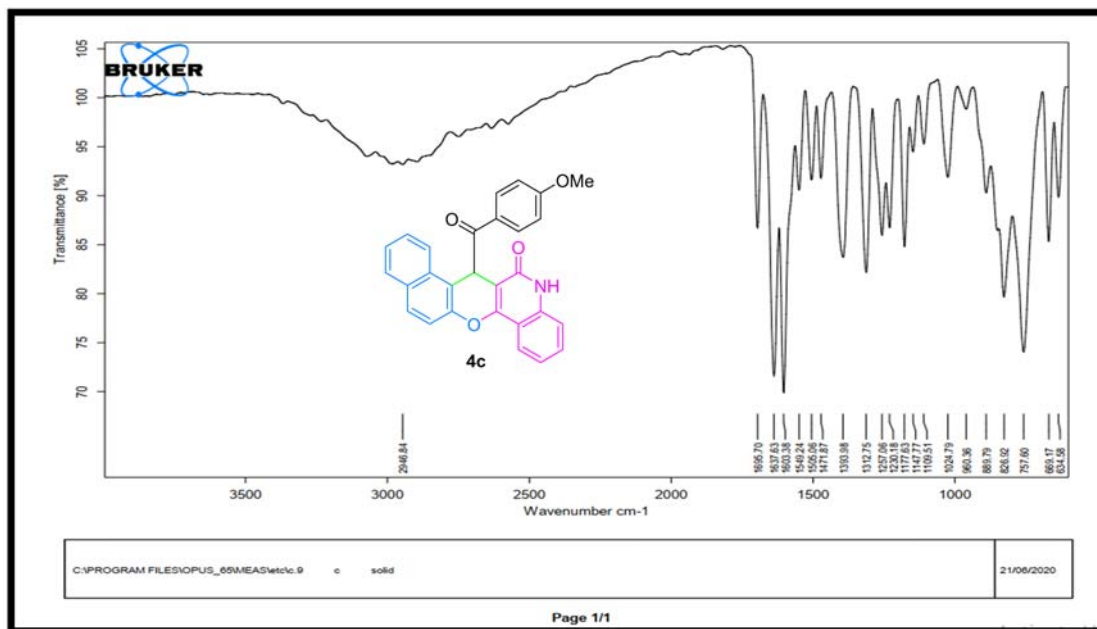
Figure S12: IR spectrum of compound 4c.
