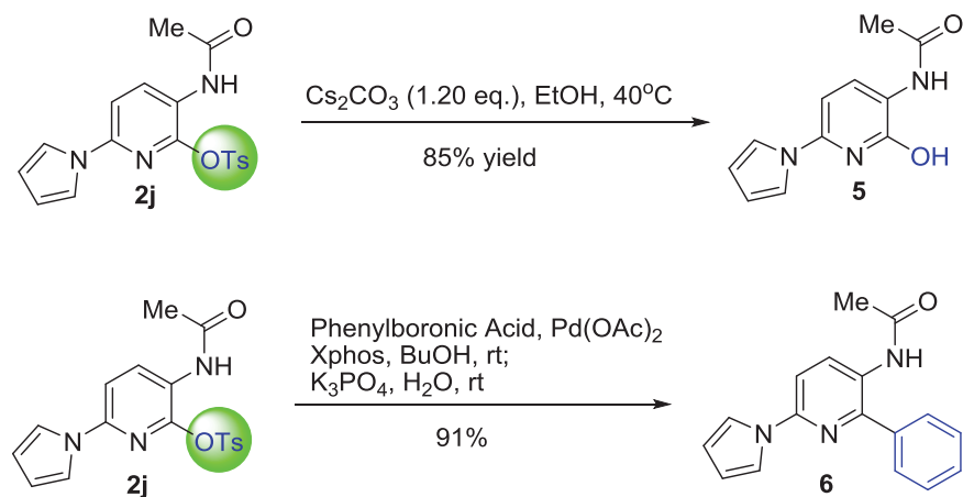
Scheme 4 Manipulation of the product.
