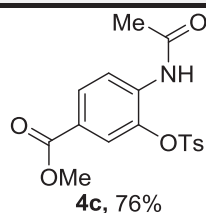
Scheme 2 Selected examples for synthesis of 2-acetamidophenyl 4-methylbenzenesulfonate under optimized conditions.
