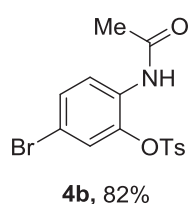
Scheme 2 Selected examples for synthesis of 2-acetamidophenyl 4-methylbenzenesulfonate under optimized conditions.
