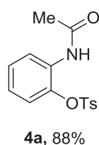
Scheme 2 Selected examples for synthesis of 2-acetamidophenyl 4-methylbenzenesulfonate under optimized conditions.
