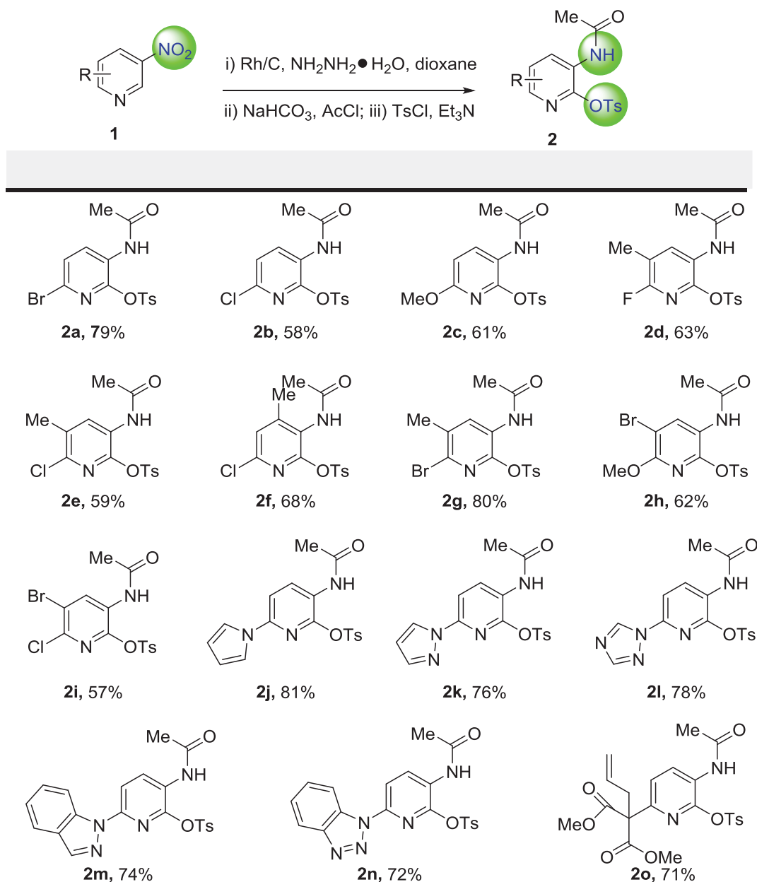
Scheme 1 Reaction scheme for synthesis of 3-acetamidopyridin-2-yl 4-methylbenzenesulfonate derivatives.
