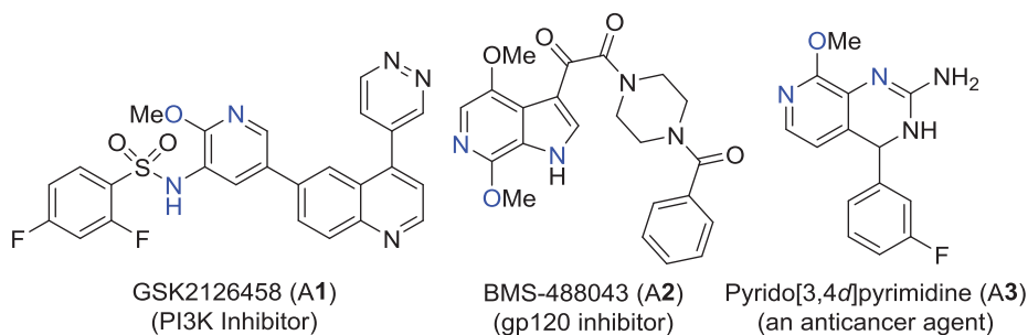
Figure 1 Selected bioactive molecules bearing the 3-amino-2-oxypyridine core structure.
