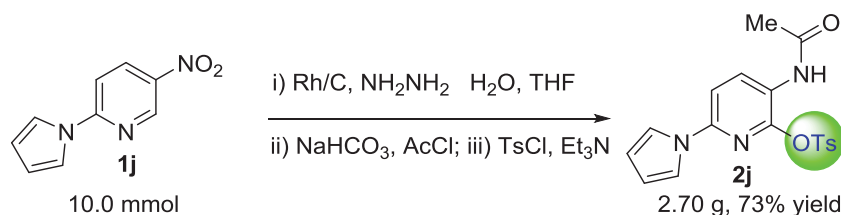
Scheme 3 Gram-Scale Synthesis of Compound 2j .
