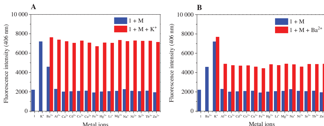
Figure 2 Panels (A) and (B) show the results of interference tests in ethanol of 1-K^+ and 1-Ba^{2+} by other metal ions. Blue bar: 1 ( 7 \mu M ) in the presence of five equivalents of another metal ion. Red bar: 1 ( 7 \mu M ) in the presence of five equivalents of K^+ or Ba^{2+} and five equivalents of another metal ion. Response of 1 ( 7 \mu M ) is included as control. The excitation was at 343 nm and fluorescence at 406 nm was measured in all cases.
