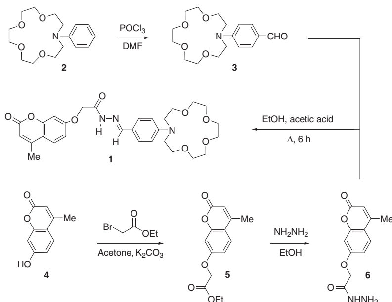
Scheme 1 The synthetic route to fluorescent sensor 1 .
