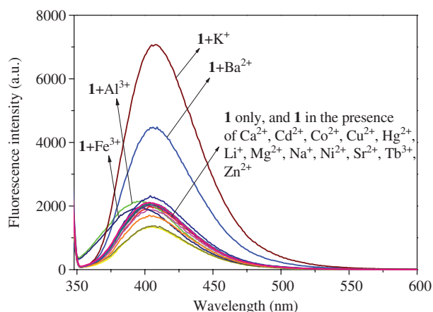
Figure 1 Fluorescence emission spectra of 1 (7 \mu\text{M} ) in ethanol in the presence of five equivalents of different metal ions ( \lambda_{\text{ex}} = 343 \text{ nm} ).
