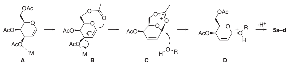
Scheme 4 Proposed mechanism to obtain galactosides 5a–d .
