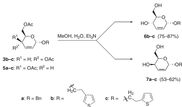
Scheme 5 Synthesis of compounds 6b–c and 7a–c .
