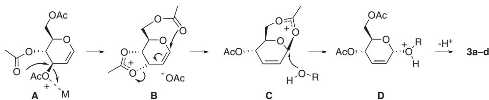
Scheme 3 Proposed mechanism to obtain glucosides 3a–d .
