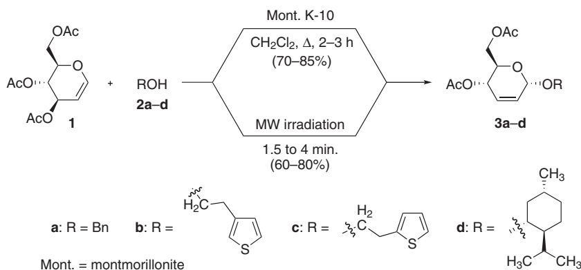
Scheme 1 Synthesis of 2,3-unsaturated O -glucosides 3a–d .
