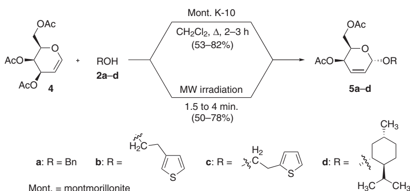
Scheme 2 Synthesis of 2,3-unsaturated O -galactosides 5a–d .
