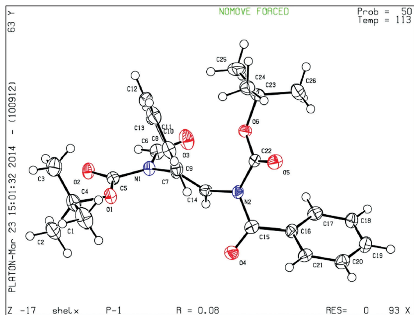
Figure 1: ORTEP diagrams of the crystal structure of 4b .
