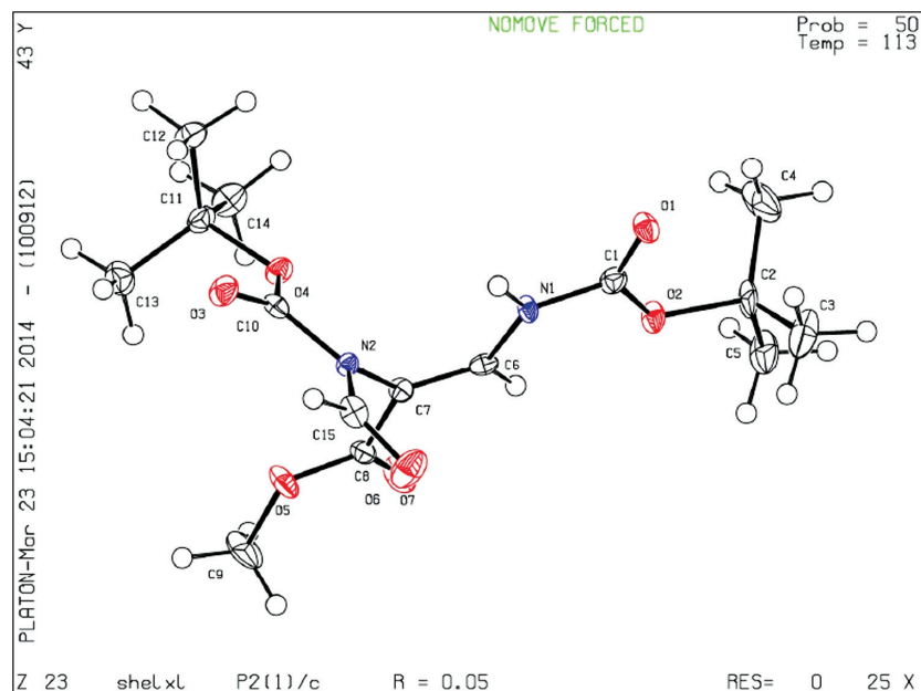
Figure 2: ORTEP diagrams of the crystal structure of 5c .
