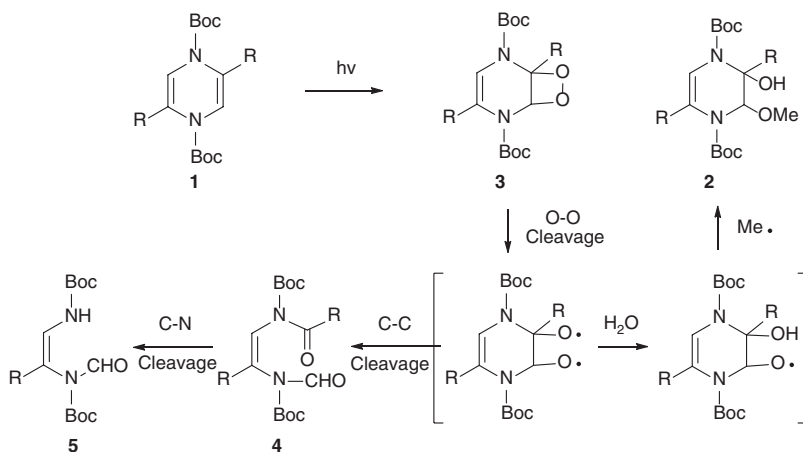
Scheme 4 Proposed mechanism for the photooxygenation of 1 .
