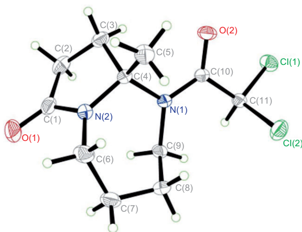
Figure 1 Structure of 4c showing 30% probability ellipsoids.
