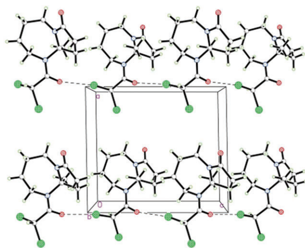
Figure 2 Packing view of 4c .
