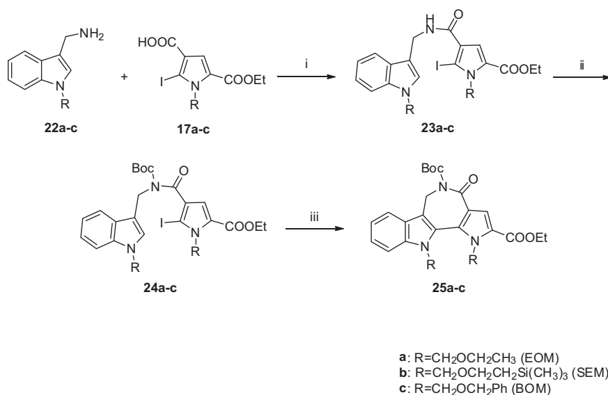
Scheme 4 Reagents and conditions: (i) EDCI·HCl, DMAP, CH 2 Cl 2 , 0°C, 4 h, then rt 19 h, R = EOM, 80%; R = SEM, 70%; R = BOM, 62%; (ii) Boc 2 O, DMAP, CH 3 CN, 21 h, rt, R = EOM, 63%; R = SEM, 63%, R = BOM, 62%; (iii) Pd(OAc) 2 , PPh 3 , Ag 2 CO 3 , DMF, 0.5 h, 135°C, R = EOM, 32%; R = SEM, 41%; R = BOM, 40%.
