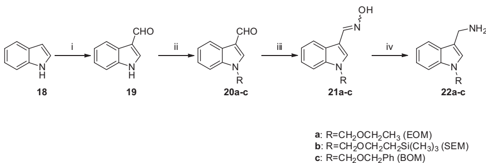
Scheme 3 Reagents and conditions: (i) (Xu and Fan, 2011) POCl 3 , DMF, 35°C, 1 h, then 20% aq. NaOH, reflux, 6 h, 96%; (ii) RCl, NaH, DMF, rt, 2 h, R = EOM, 89%; R = SEM, 98%; R = BOM, 98%; (iii) H 2 NOH·HCl, Na 2 CO 3 , C 2 H 5 OH/H 2 O, reflux, 2–5.5 h, R = EOM, 95%; R = SEM, 89%; R = BOM, 96%; (iv) NiCl 2 ·6H 2 O, NaBH 4 , MeOH, rt, 10 min, R = EOM, 100%; R = SEM, 60%; R = BOM, 93%.
