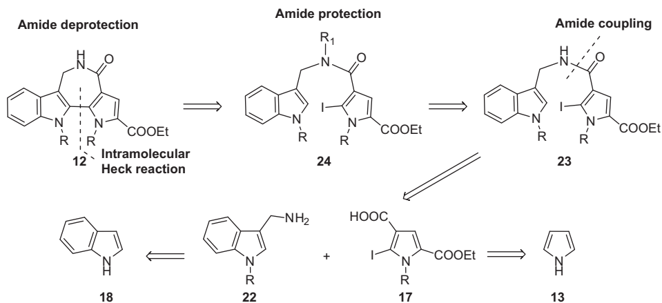
Scheme 1 Retrosynthetic analysis of the new tetracyclic core 12 .
