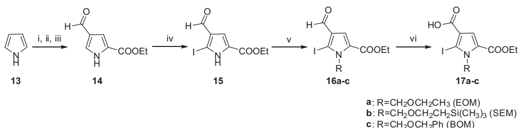
Scheme 2 Reagents and conditions: (i) (Bailey et al., 1971) (1) Cl 3 CCOCl, (C 2 H 5 ) 2 O, rt, 1 h (2) K 2 CO 3 , H 2 O, 79%; (ii) (Bailey et al., 1971) Na/C 2 H 5 OH, rt, 0.5 h, 91%; (iii) (Garrido et al., 1988) Cl 2 CCH 2 OCH 3 , AlCl 3 , CH 2 Cl 2 /CH 3 NO 2 , -20°C, 18 h, 80%; (iv) (Farnier and Fournari, 1973) I 2 , HIO 3 , H 2 SO 4 , CH 3 COOH/H 2 O/CCl 4 , 5 h, 80°C, 33%; (v) RCl, NaH, DMF, rt, 2 h, R = EOM, 95%; R = SEM, 94%; R = BOM, 70%; (vi) KMnO 4 , acetone/H 2 O, rt, 5.5 h, R = EOM, 80%; R = SEM, 50%; R = BOM, 80%.
