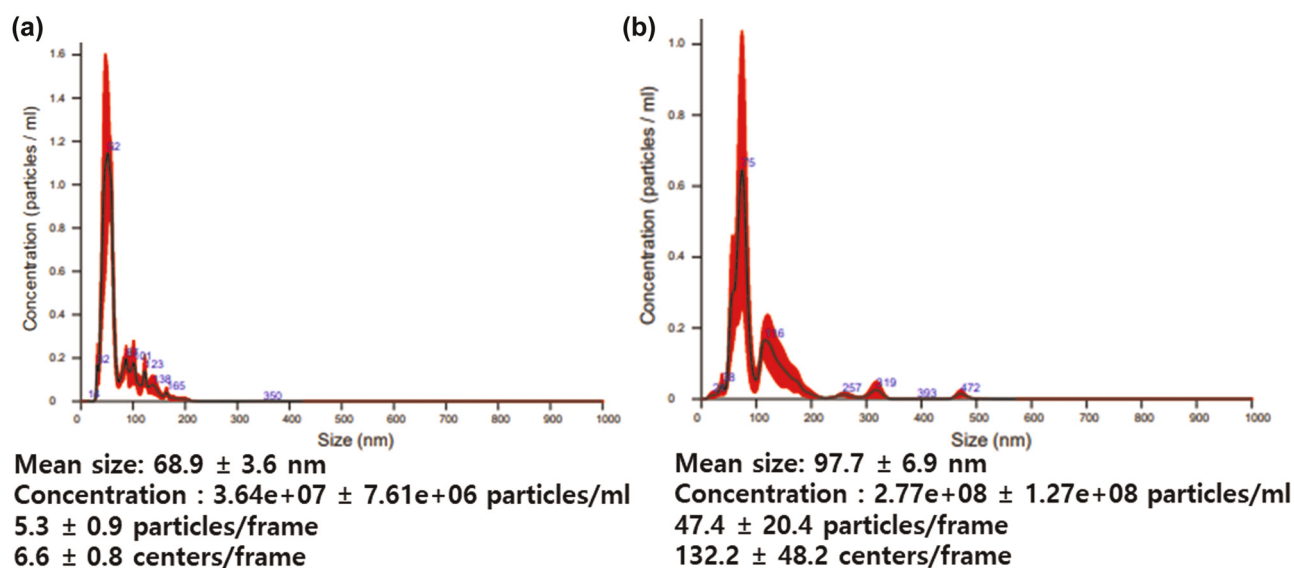
Figure S1: PLE-AgNPs concentration was analyzed and compared to AgNO 3 solution at equal concentration using a nanoparticle tracking analyzer (NTA).
