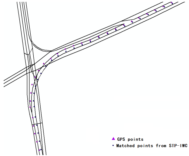
Figure 8: Test case of STP-IWC algorithm
