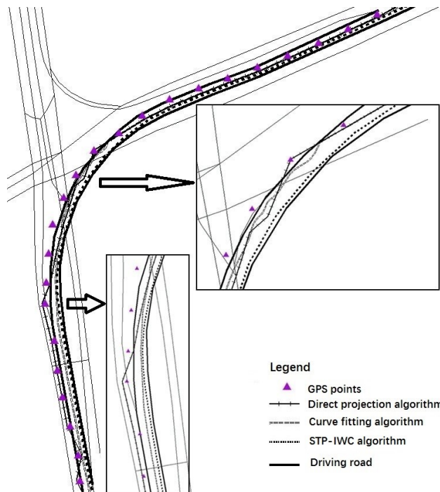
Figure 9: Matching results from different algorithms
