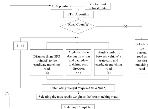
Figure 5: STP-IWC algorithm
