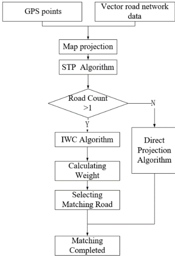
Figure 1: Overall process of STP-IWC algorithm
