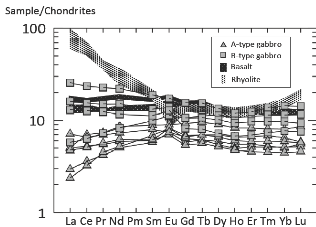
Figure 6: Rare earth element (REE) variation diagrams for xenoliths and volcanic rocks from Niiijima volcano. REE data were normalized to C1 chondrite [33]. Basaltic inclusion data from Atchiyama rhyolite are nearly the same with basalt data in Wakago. Most of the data of rhyolites in Niiijima are referred from [23, 32] and shown (light-shaded area).
