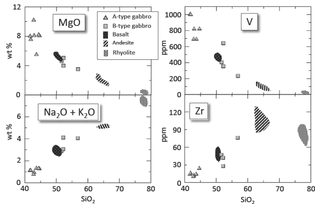
Figure 5: Comparison of selected major and trace elements for the two types of gabbro and host rocks from Niiijima volcano. Andesite data from Shimawakezawa pyroclastic unit and some data of the basaltic mafic inclusions are from the Atchiyama rhyolite from Endo [23]. Some of the basalt and andesite data are used from Isshiki [16].
