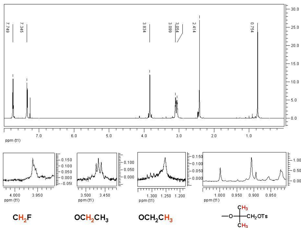
Fig. 3. ^1\text{H} -NMR spectra of pTMMO1-BDO. \delta (ppm): 7.75-7.34 ppm (aromatic protons of Ts), 4.15-4.13 (end OH(acetylated)- TMMO), 3.83 ( \text{CH}_2\text{OTs} ), 3.10 ( \text{CH}_2\text{O-TMMO} ), 2.41 (arylic \text{CH}_3 - TMMO), 0.75 ( \text{CH}_3 -TMMO).
