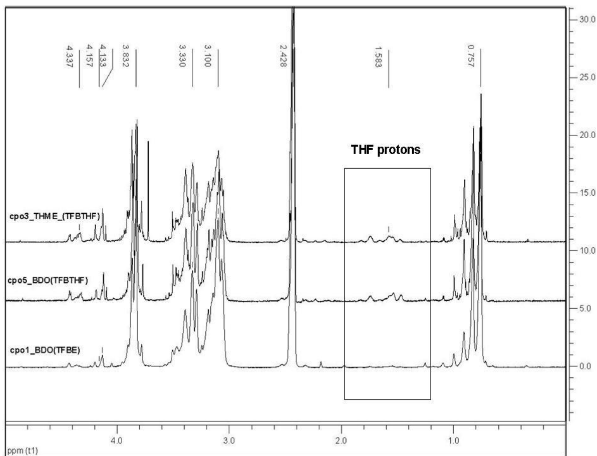
Fig. 5. ^1\text{H} -NMR spectra of TMMO-co-BBrMO: \delta (ppm) 4.34 (end OH(acetylated)-BBrMO), 4.15-4.13 (end OH(acetylated)- TMMO), 3.83 ( \text{CH}_2\text{OTs} ), 3.33( \text{CH}_2\text{-BBrMO} ), 3.10 ( \text{CH}_2\text{O-TMMO} ), 2.43 (arylic \text{CH}_3\text{-TMMO} ), 1.58 ( \text{CH}_2\text{-THF} ), 0.76 ( \text{CH}_3\text{-TMMO} ).
