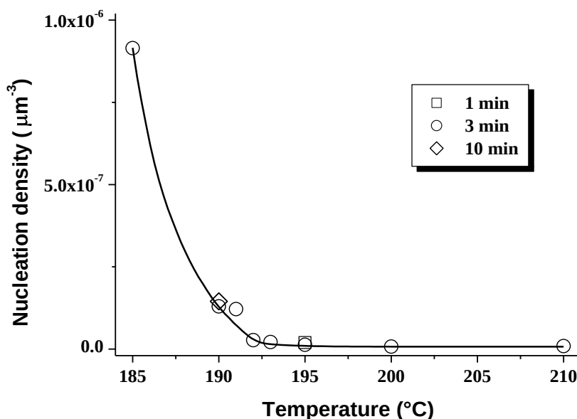
Fig. 6. Nucleation density of PHB after completion of crystallization at 5 °C/min as a function of temperature of preceding thermal treatment for the indicated times.
