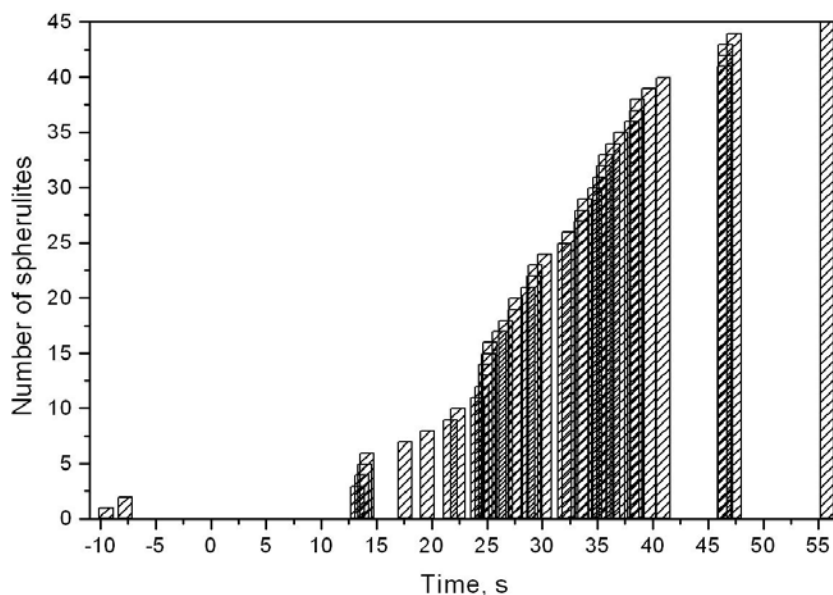
Fig. 1. Number of shperulites vs. time during crystallization at 92 °C.
