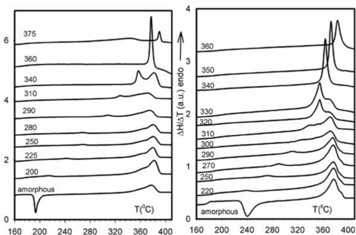
Fig. 6. DSC heating curves recorded at 10 \text{ }^{\circ}\text{C/min} for amorphous samples of PEKEKK annealed for 30 min at different temperatures (left) and amorphous samples of 2,6-PEKEKNK annealed for 1 hr (right) after heating at 10 \text{ }^{\circ}\text{C/min} .
