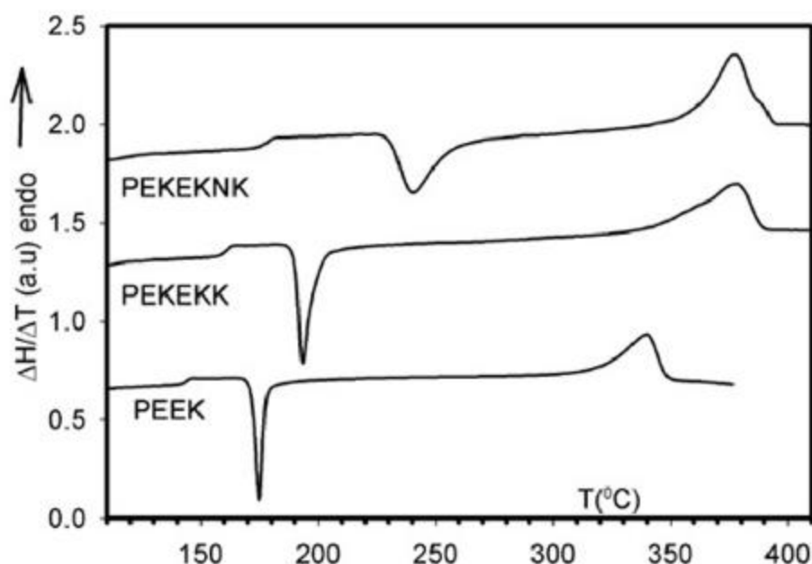
Fig. 5. DSC heating curves recorded at 10\text{ }^{\circ}\text{C/min} for amorphous PEEK, PEKEKK and PEKEKNK.
