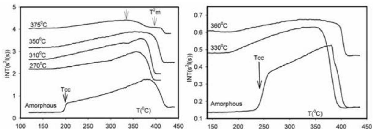
Fig. 11. Evolution of the integrated SAXS intensity for 0.02 \leq s \leq 0.2 nm -1 during heating scans at 10 °C/min of an amorphous sample and samples annealed at different temperatures for PEKEKK (left) and PEKEKNK (right). Note the jump in intensity at the cold crystallization temperature ( T_{cc} ) of the amorphous sample. Note also the broad feature around 340 °C and melting at T_m^2 = 390 °C for the PEKEKK sample annealed at 375 °C as also observed in the DSC traces in Fig. 6 (left). For the amorphous 2,6- PEKEKNK sample compare the shoulder around 388 °C with that in the DSC trace in Fig. 5.
