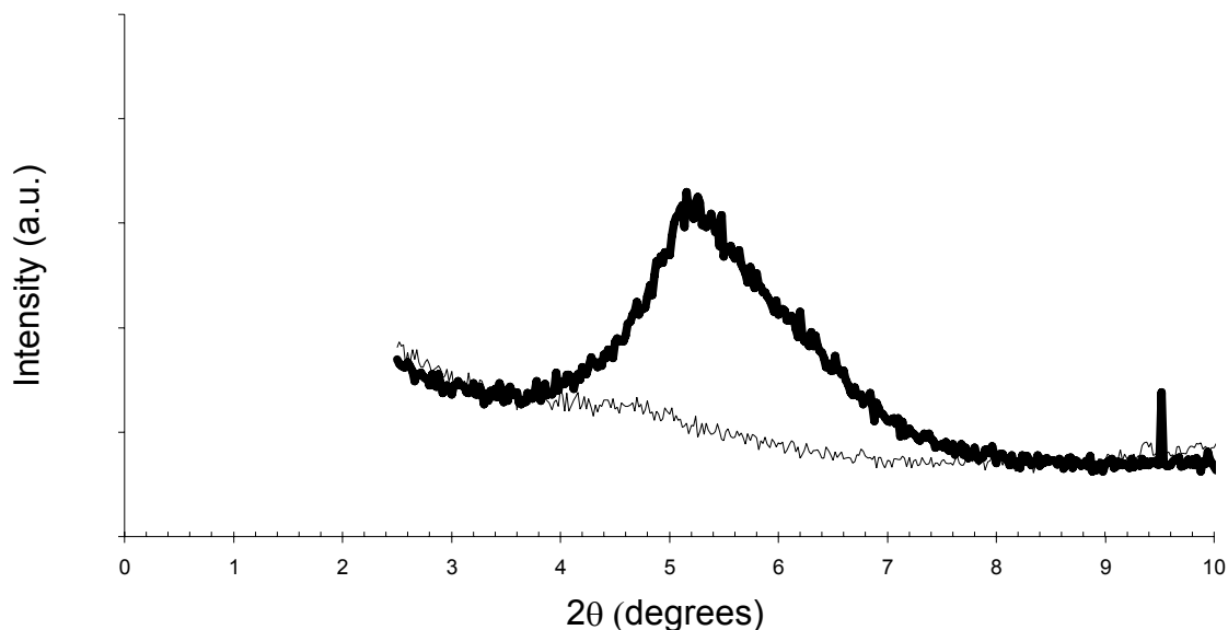
Fig. 1. X-ray diffraction patterns of Nanofil 784® (—) and nanocomposite sample PA6N784(3) (---) from 2.5^\circ to 10^\circ of 2\theta .
