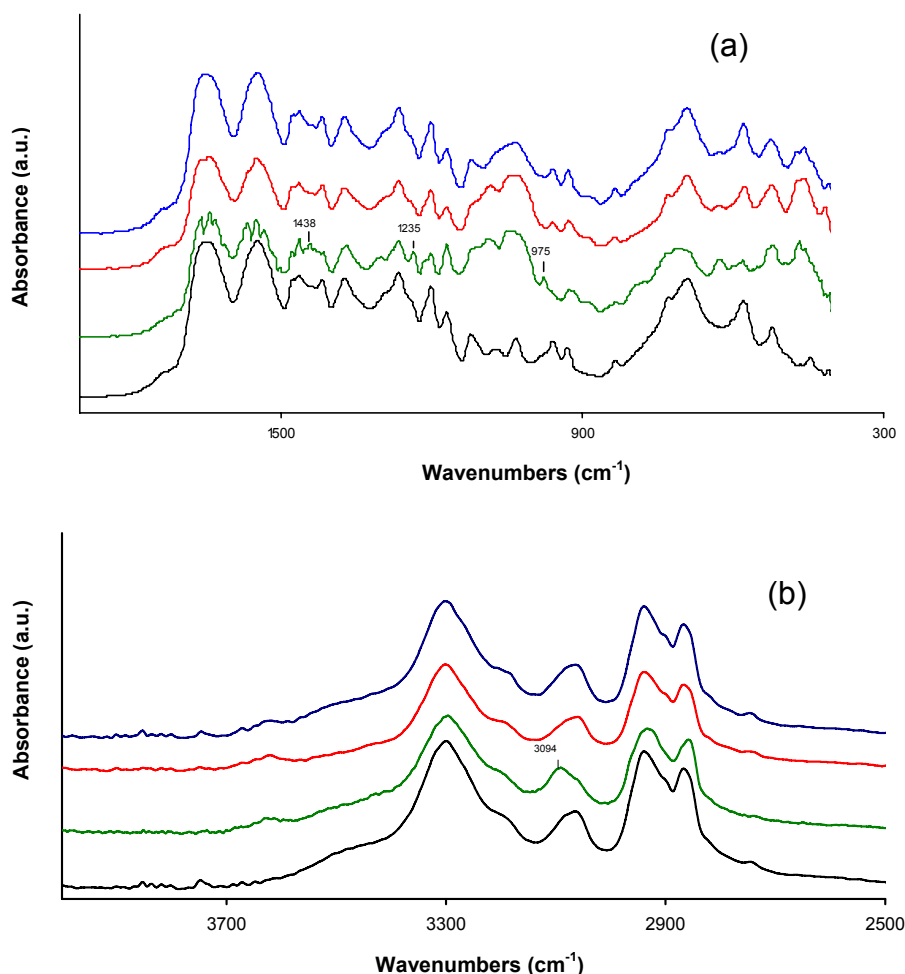
Fig. 7. FTIR spectra of neat PA6 (—) and nanocomposite samples PA6ClNa(1) (PA6/Cloisite Na ® ) (—), PA6N784(3) (PA6/Nanofil 784 ® ) (—) and PA6Cl30B(1) (PA6/Cloisite 30B ® ) (—).
