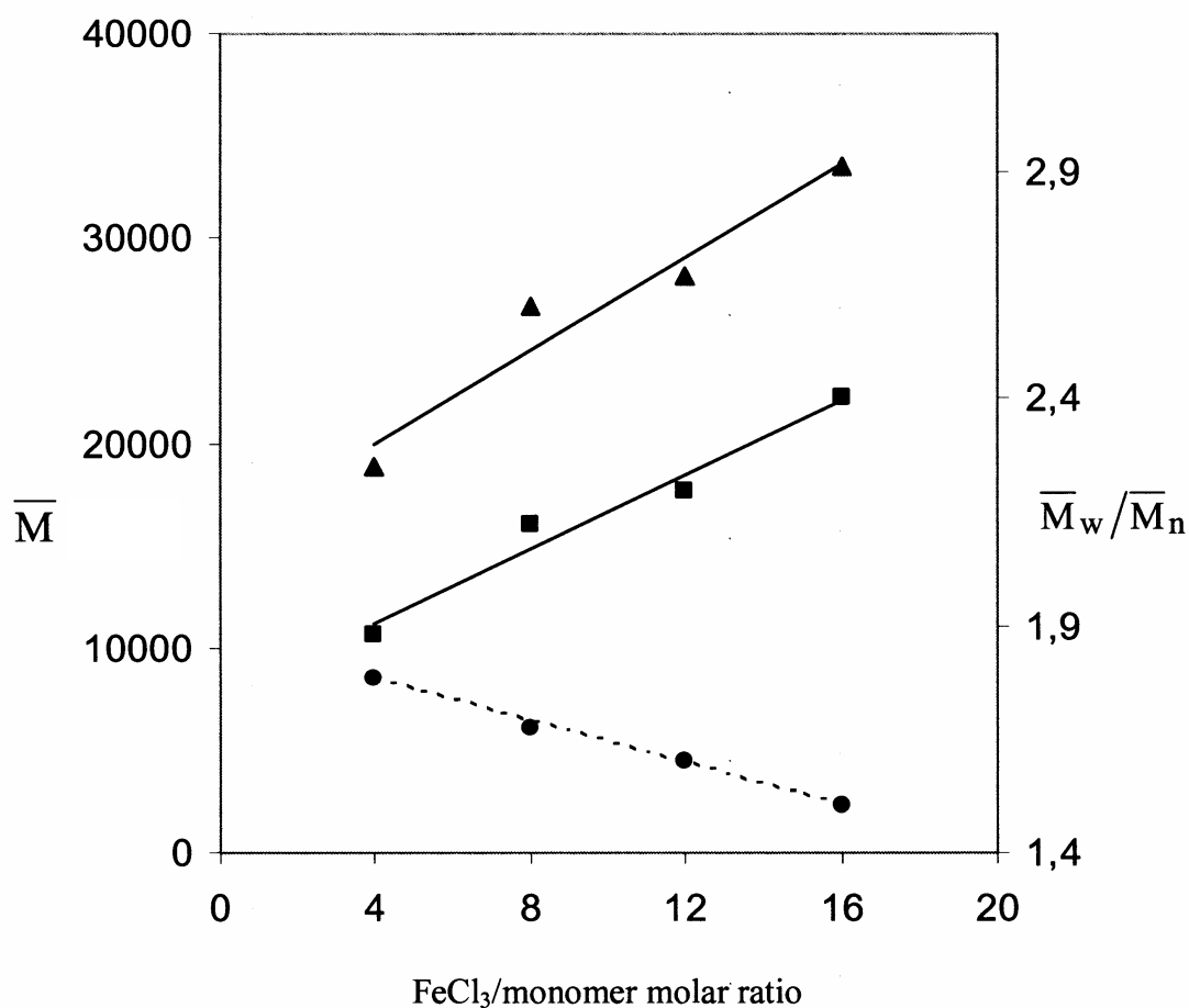
Fig. 2. Variation of \overline{M}_w (▲), \overline{M}_n (■) and \overline{M}_w/\overline{M}_n (●) with the \text{FeCl}_3/\text{monomer} molar ratio in the synthesis of poly(DDDMBQT).
