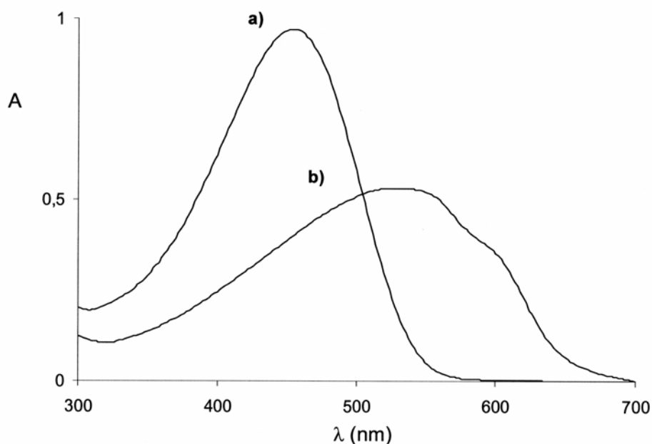
Fig. 3. UV-vis spectra of poly[( S )-(+)-DDDMBQT] 2.3 \cdot 10^{-5}\text{ M} in chloroform (a) and chloroform/methanol 40/60 v/v solution (b).
