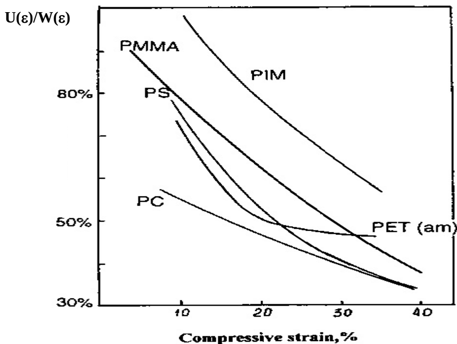
Fig. 4. Ratio U(\varepsilon) / W(\varepsilon) for different glassy polymers for strains \varepsilon_{def} \geq \varepsilon_y [4, 26]. T_{def} = room temperature.
