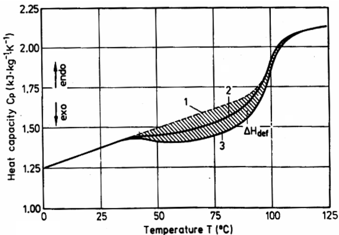
Fig. 6. DSC traces for glassy PS deformed in different ways [38]. Heating rate - 20 deg/min. 1- Non-deformed sample. 2- Uniaxial tension, \varepsilon_{res} = 3\% . 3-Uniaxial compression, \varepsilon_{res} = 30\% . T_{def} = room temperature.
