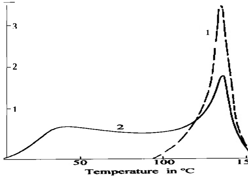
Fig. 7. Thermally stimulated \epsilon_{\text{res}} recovery curves for EAAN deformed at different temperatures. 1- T_{\text{def}} = 160^{\circ}\text{C} , \epsilon_{\text{res}} = 17\% . Deformed sample was cooled then to room temperature with fixed length ( \epsilon_{\text{res}} constant). 2- T_{\text{def}} = \text{room temperature} . \epsilon_{\text{res}} = 20\% . Recovery rate \dot{\epsilon}_{\text{res}} – in %/min. Heating rate – 20 deg/min [16].
