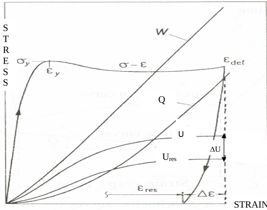
Fig. 2. Variations of W(\epsilon) , Q(\epsilon) , U(\epsilon) , U_{res}(\epsilon) and \Delta U(\epsilon) at loading and unloading of glassy polymers (see text) [38]. \Delta\epsilon —amount of strain relaxed during sample unloading at T_{unl} . \sigma_y and \epsilon_y —yield stress and strain. \epsilon_{res} —residual strain, \Delta\epsilon = \epsilon_{an} + \epsilon_{pl} + \epsilon_{vp} (see Fig.1). \Delta U —elastic energy collected by sample.
