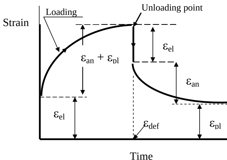
Fig. 1. Components of total strain \epsilon_{\text{def}} accumulated by a solid sample at it's loading by a constant stress and the disappearance of the components after unloading. T_{\text{def}} = \text{const} . The following relations are valid: \epsilon_{\text{el}} = \epsilon_{\text{le}} + \epsilon_{\text{nle}} , where \epsilon_{\text{le}} is linear-elastic and \epsilon_{\text{nle}} – nonlinear-elastic components; \epsilon_{\text{pl}} –plastic component; \epsilon_{\text{pl}} = \epsilon_{\text{res}} \text{ apparent} = \epsilon_{\text{conf}} + \epsilon_{\text{vp}} below T_g . In polymers \epsilon_{\text{conf}} is conformational and \epsilon_{\text{vp}} is visco-plastic components. \epsilon_{\text{an}} is anelastic (delayed elastic) component [1]. \epsilon_{\text{an}} exists only in the solid state of matter, i.e. below T_g or T_m . \epsilon_{\text{pl}} is the component able to recover only in the liquid (rubbery) state of matter, i.e. at T \geq T_g ( T_m ).
