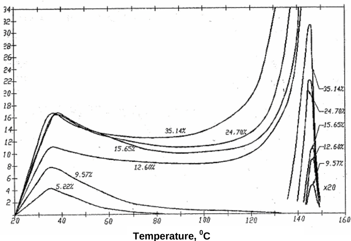
Fig. 8. Thermally stimulated rate recovery curves for PC deformed at 20°C up to different strain levels. Numbers on curves show amount of strain \epsilon_{res} for each sample ( T_{def} = RT ). Amount of \epsilon_{def} \approx (\epsilon_{res} + 5-7\%) . Heating rate – 20deg/min. Intensity of recovery peaks at T_g multiplied x20.
