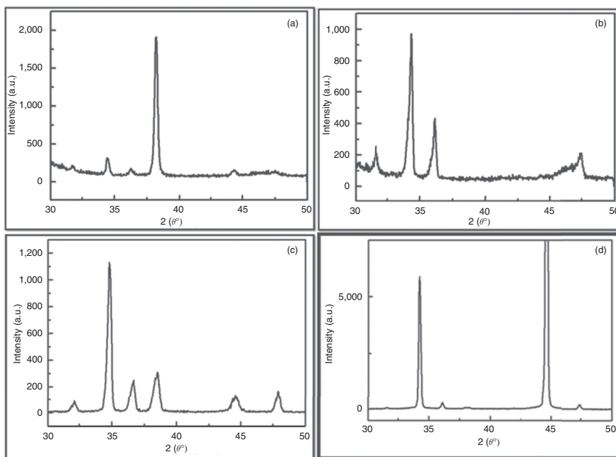
Figure 3 XRD spectra of ZnO NRs grown on (a) common paper, (b) plastic, (c) textile fabric and (d) aluminum foil
