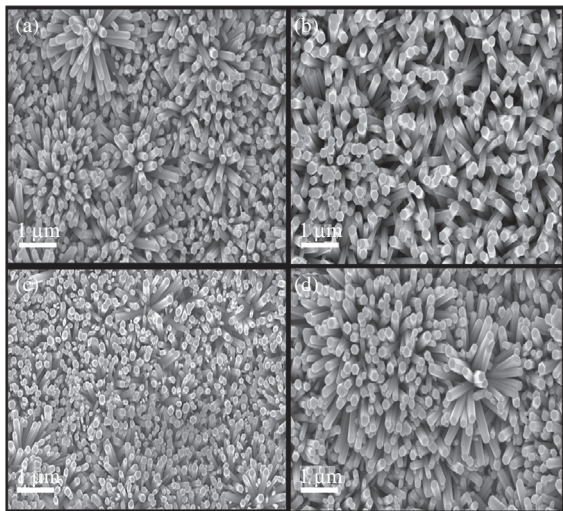
Figure 2 The SEM images of ZnO NRs grown on different flexible substrates. (a) Common paper, (b) plastic, (c) textile fabric and (d) aluminum foil
