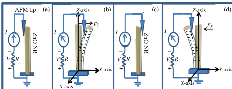
Figure 4 Schematic diagram showing the mechanism of the electrical pulse generation by ZnO NRs
