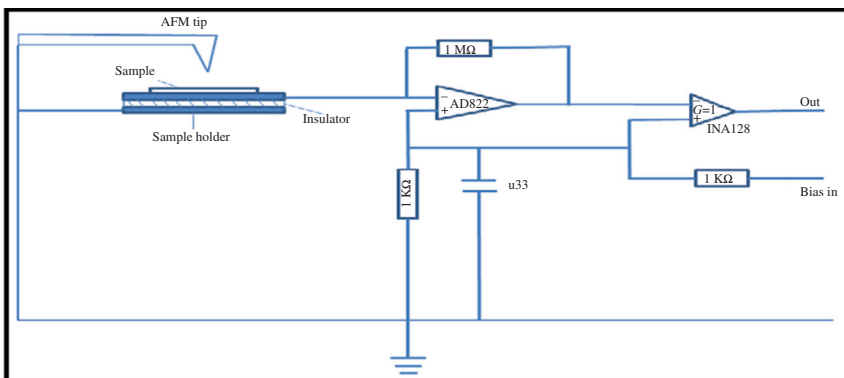
Figure 1 Schematic diagram showing the current-amplifier circuit
