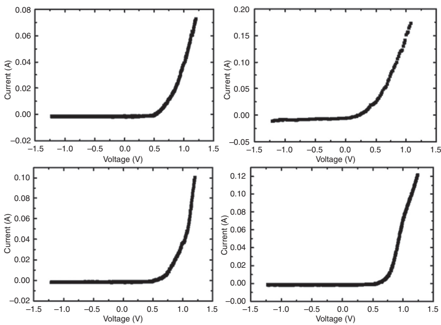
Figure 6 I - V characteristics for (a) common paper, (b) plastic, (c) textile fabric and (d) aluminum foil
