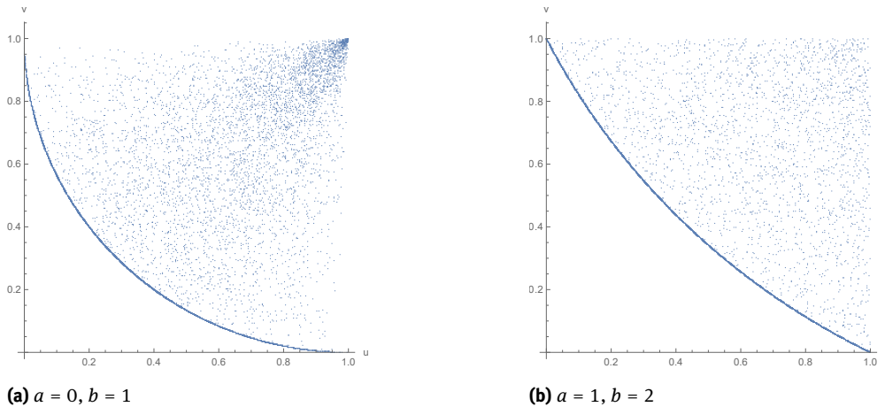
Figure 12: Two simulations from a uniform Lorenz copula with X \sim U[0, 1] and X \sim U[1, 2] .
