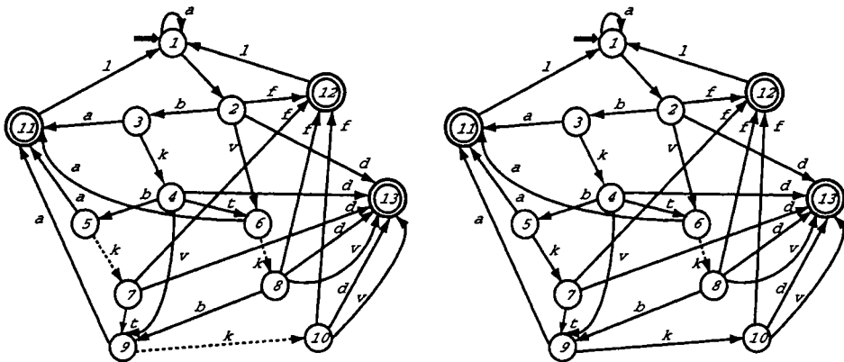
(a) Supervision without Event Disabling Cost (b) Supervision with Event Disabling Cost
