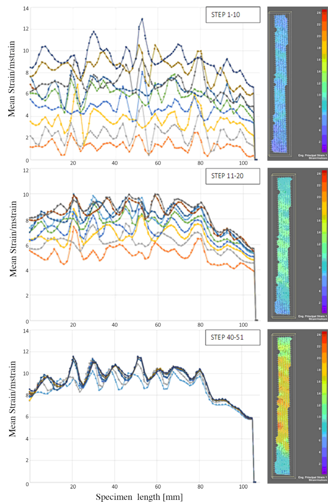
Figure 9: Strain vs Time in different steps. Specimen F5(30)
