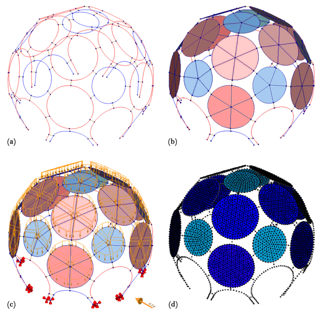
Figure 14: Diana FEA setting phases: (a) Model with all the directions of the structural elements is presented: in red, the hexagon's beams; in blue, pentagonal beams; in black, the junctions; (b) insertion of the infilling surfaces; (c) Complete DIANA model with the application of the snow load and the seismic actions; (d) Output of the calculus obtained by the software
