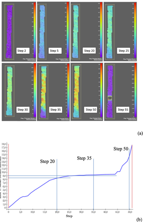
Figure 8: Mean strain versus steps (Time graph). The specimens were subjected to a tensile test until the collapse conditions were reached. Specimen F5(30)
