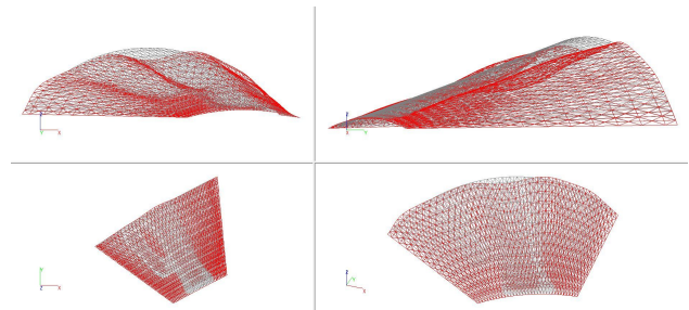
Figure 13: The deformation scheme of conoid shell
