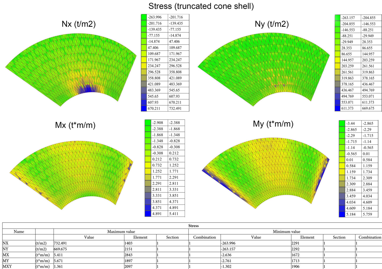
Figure 11: The normal stresses of the truncated cone shell
