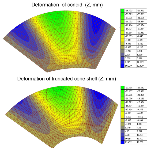
Figure 15: The z-axis deformation
