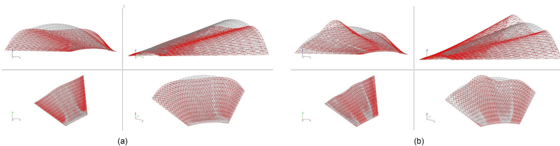
Figure 7: The deformation scheme of conoid shell
