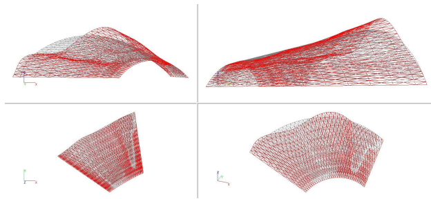
Figure 14: The deformation scheme of truncated cone shell
