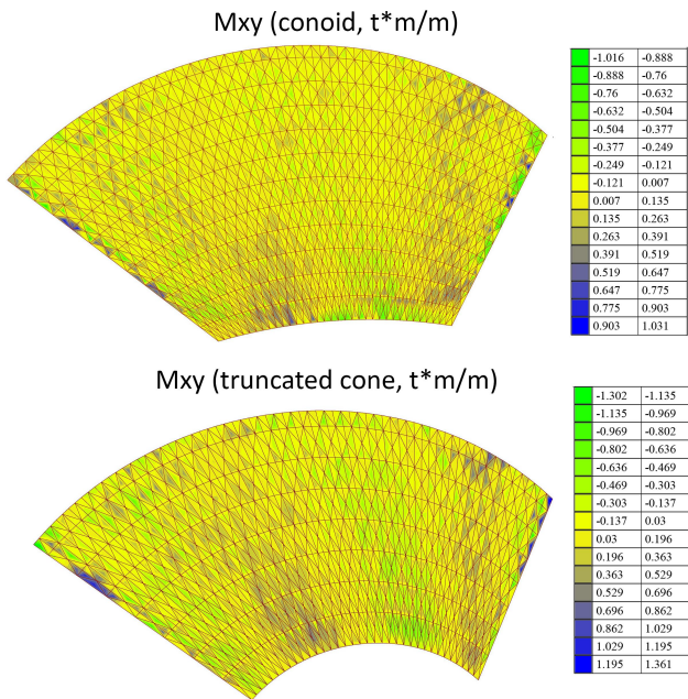
Figure 12: The Mxy parameter of the two shells
