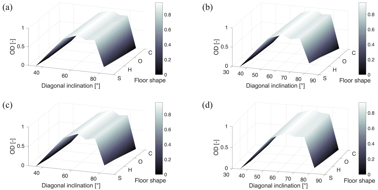
Figure 4: Surface representation of the OD with respect to the diagrid geometrical parameters obtained with different combinations of the individual desirability exponents: (a) r_\delta = 2.00 , r_\phi = 1.00 , r_M = 1.00 , r_{CI} = 1.00 ; (b) r_\delta = 1.50 , r_\phi = 0.75 , r_M = 1.25 , r_{CI} = 1.00 ; (c) r_\delta = 1.50 , r_\phi = 1.00 , r_M = 1.00 , r_{CI} = 1.25 ; (d) r_\delta = 2.00 , r_\phi = 1.25 , r_M = 1.75 , r_{CI} = 0.75
